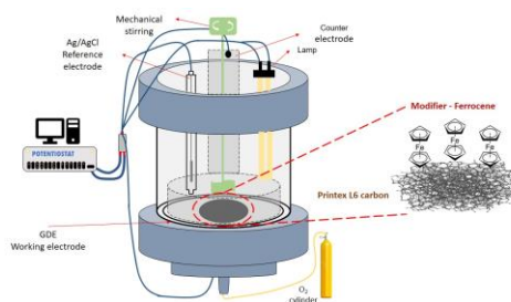
Figure 1. Schematic diagram of the three-electrode cell used to evaluate the three different prepared GDEs for electrosynthesis of H 2 O 2 and degradation of PCT.
