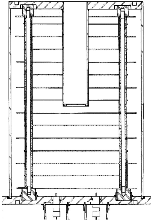
Fig. 2. Longitudinal section of the cylindrical ionization chamber with parallel electrodes.
