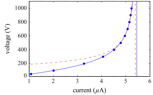
Fig. 5. Measured I – \Delta V characteristic curve with a radioactive source of 55 Ci. The resulting saturation current was I_{sat} = 5.45 \mu A, in the case of the estimate based on the exact solution, and I_{sat} = 5.40 \mu A in the other case, yielding a relative deviation of 1%. The legend is the same as in Fig. 4.
