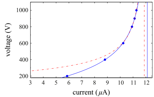
Fig. 6. Measured I – \Delta V characteristic curve with a radioactive source of 120 Ci. The resulting saturation current was I_{sat} = 12.11 \mu A, in the case of the estimate based on the exact solution, and I_{sat} = 11.88 \mu A in the other case, yielding a relative deviation of 2%. The legend is the same as in Fig. 4.
