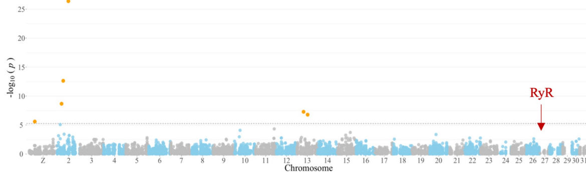
Fig 1. Genome-wide association plot of single nucleotide polymorphisms associated with flubendiamide survival traits in field-derived Helicoverpa armigera . The x-axis denotes the number and position of markers across chromosomes. The y-axis illustrates the -\log_{10}(p) values to depict the significance of each SNP. A horizontal dashed line indicates the Bonferroni-adjusted significance threshold of 5.4 \times 10^{-6} . A red arrow identifies the location of the ryanodine receptor gene on the H. armigera reference genome.
