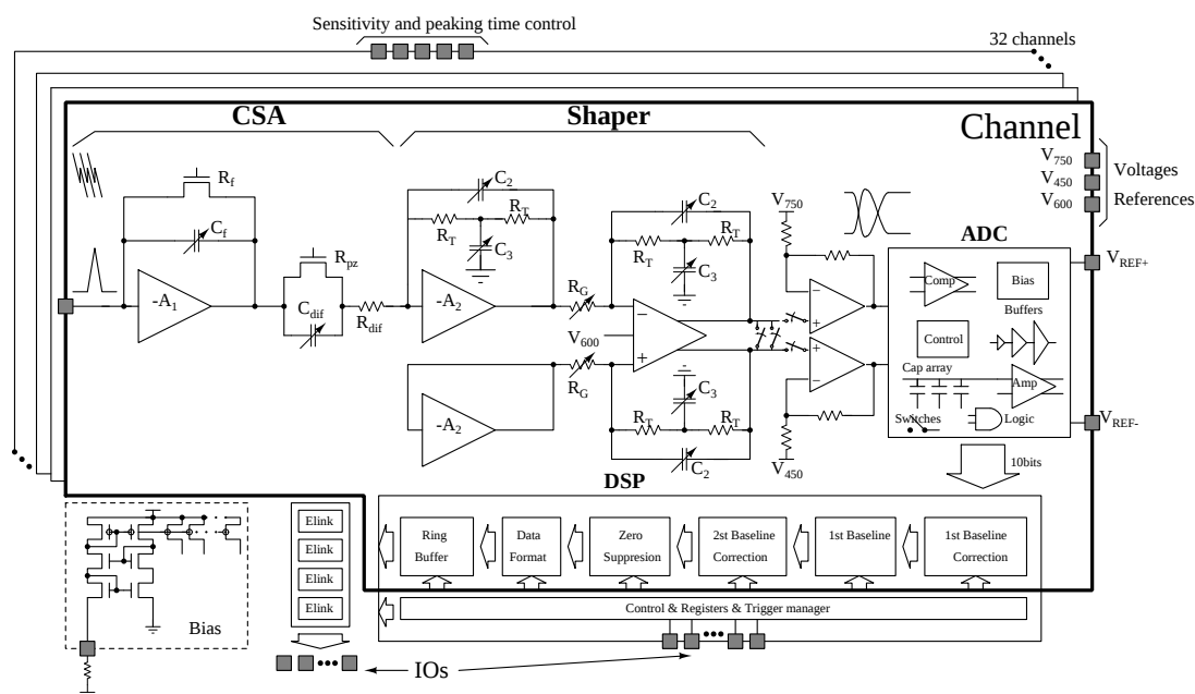
Figure 1. Sampa block diagram.
