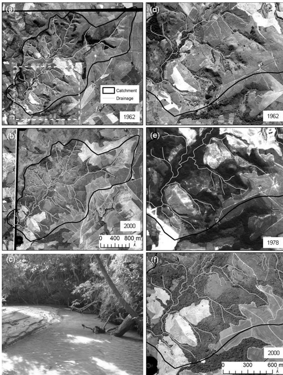
Fig. 4. Forest cover regeneration and stream sedimentation in an agricultural landscape. Forest cover regeneration in the last decades (A-B – the regenerated area represented by the white dotted square is shown in detail in D-F). Channel completely filled with sand in the sampled reach (C).
