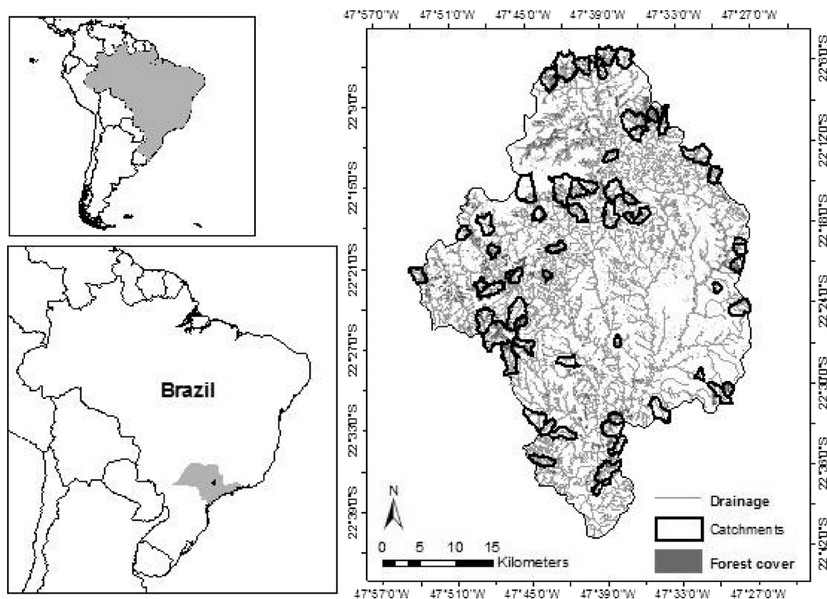
Fig. 1. Location of the 60 study sites in the Corumbataí River basin, São Paulo State, Brazil.
