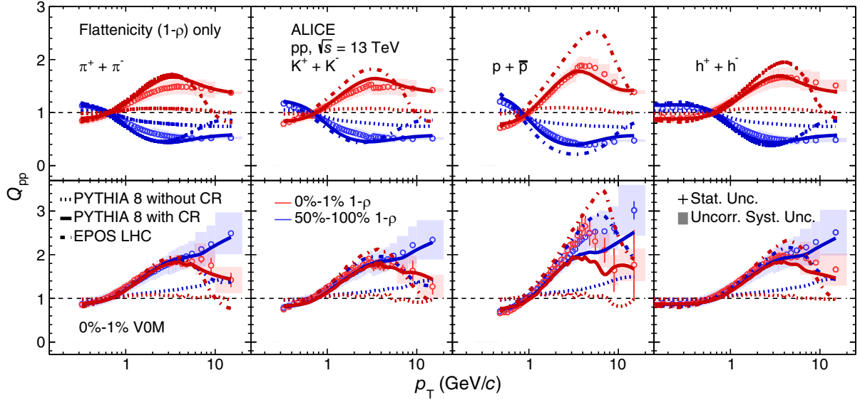
FIG. 5. The Q_{pp} ratio of \pi , K , p , and h^\pm for the 0%–1% and 50%–100% 1-\rho classes (top row) and for the same 1-\rho classes in HM (0%–1% VOM) events (bottom row). The data are compared with PYTHIA 8 and EPOS LHC model predictions. The statistical and systematic uncertainties are represented with bars and shaded areas.
