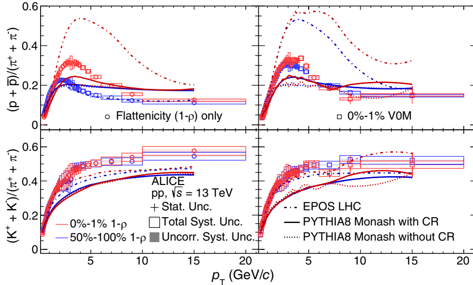
FIG. 6. The p_T -differential proton-to-pion (top row) and kaon-to-pion (bottom row) particle ratios for two extremes of flattonicity event classes, as indicated in the legends, are shown. Left and right columns include results for multiplicity-integrated and 0%–1% VOM event classes. The statistical, total, and uncorrelated systematic uncertainties are represented with bars, boxes, and shaded areas around the data points, respectively. The shaded regions around the model line represent the statistical uncertainties.
