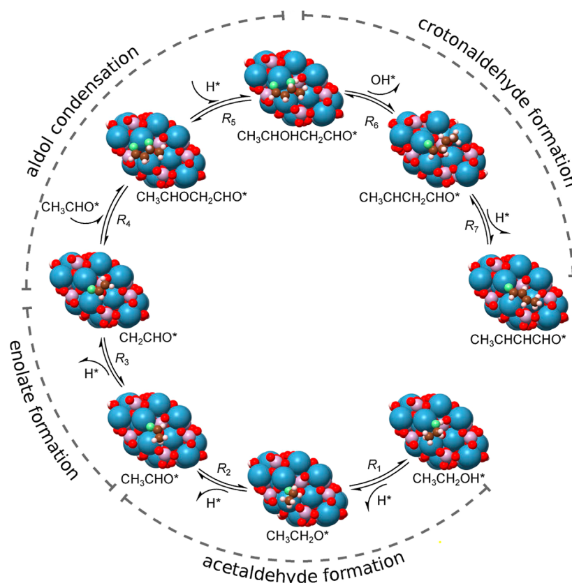
Figure 2. Proposed sequence of elementary reactions for obtaining crotonaldehyde on the HAP(0001) surface. The proposed reaction pathway encompasses the acetaldehyde formation ( R_1 and R_2 ), the enolate formation ( R_3 ), the aldol condensation ( R_4 and R_5 ), and the crotonaldehyde formation ( R_6 and R_7 ). All reactions are detailed in Table 1.
