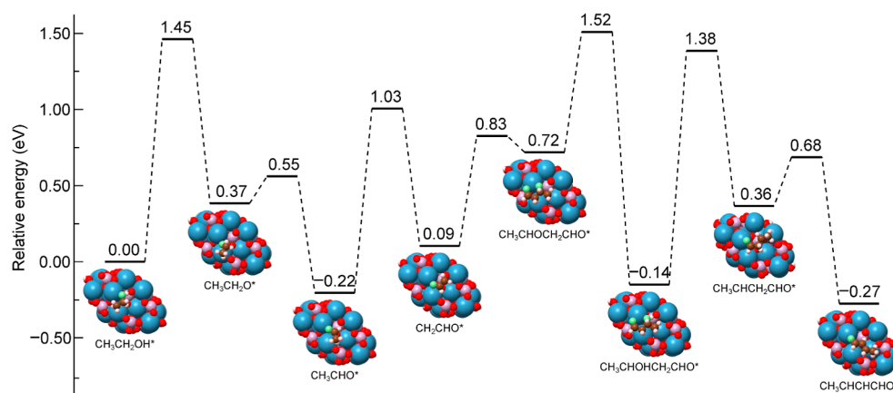
Figure 3. Free energy diagram for the proposed catalytic formation of crotonaldehyde from ethanol at 573.15 K.
