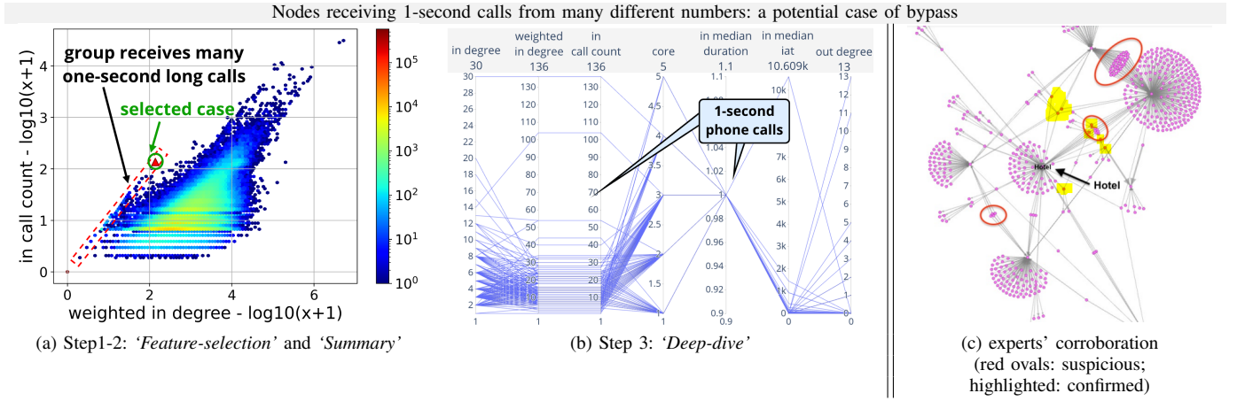
Fig. 1. TgraphSpot at work: (a) several nodes are on the 45-degree line (red dashed box), away from the majority (notice that both axes, as well as the color-scale, are in log). (b) 'Deep-dive' for the red triangle: parallel axis plot of the EgoNet of the 'red triangle', shows that the nodes receive 1-second phone calls (c) experts are investigating the nodes like the ones in red ovals, and confirmed that the callers in yellow-highlight have all the evidence of 'International Bypass' type of fraud - see text.
