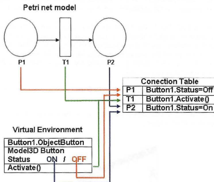
Figure 3. Link between Petri net and object
