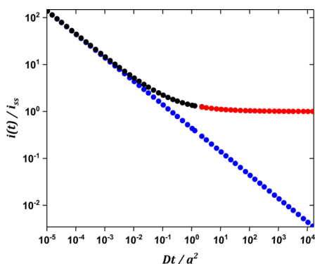
Figure 1. Current values calculated using the Cottrell equation (blue dots), and the Mahon and Oldham equation for short times (black dots) and for long times (red dots). D = 5 \times 10^{-6} \text{ cm}^2 \text{ s}^{-1} and a = 12.5 \times 10^{-4} \text{ cm} .
