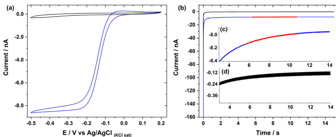
Figure 2. a) Voltammogram recorded with a 14.1 \mu\text{m} radius carbon fiber disc microelectrode in a 1.8 mmol \text{L}^{-1} hexaammineruthenium(III) + 0.1 mol \text{L}^{-1} KCl solution. Scan rate = 20 \text{mV s}^{-1} . The black line corresponds to the background CV recorded in the supporting electrolyte. b) Chronoamperogram recorded with the same microelectrode in the same solution when stepping from 0.0 V to -0.4 V. Inset: c) magnification of the current region (red) used to derive D and c , and d) magnification of the background current.
