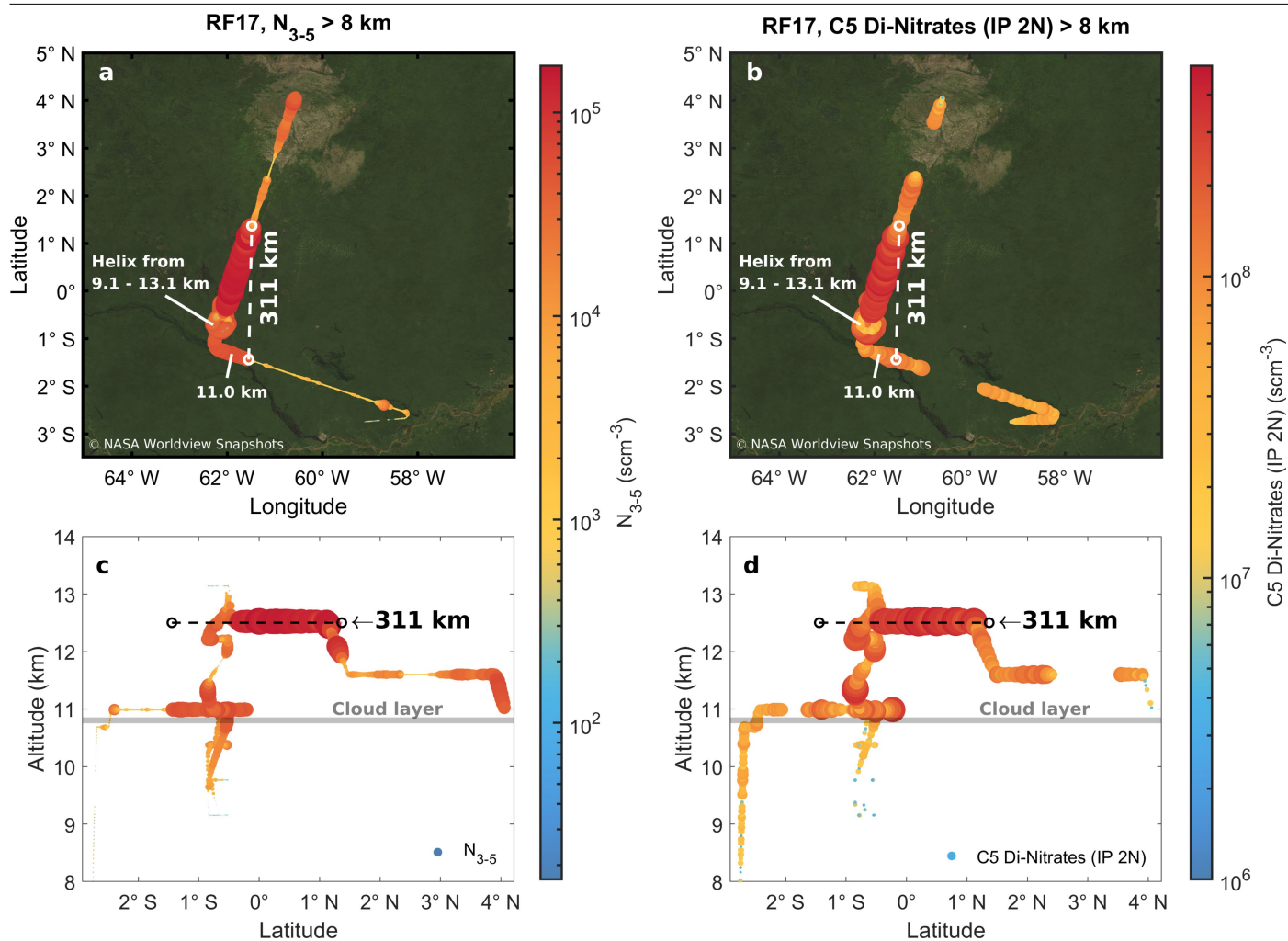
Extended Data Fig. 8 | Spatial extent of the NPF event observed during RF17, measured in the morning of 18 January 2023. a, Continuously high concentrations of N_{3-5} particles are detected in an area with an extent of more than 300 km in two layers between 10.6–11.5 and 12.0–12.6 km. A cirrus cloud deck was present at altitudes below 10.8 km. b, High concentrations of
