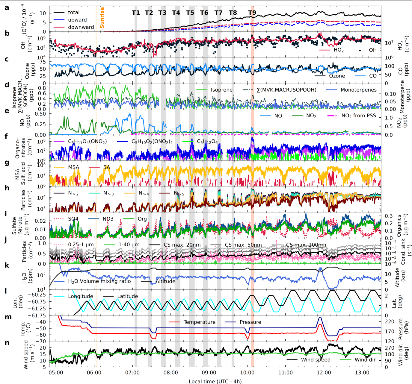
Extended Data Fig. 2 | Extended dataset for RF19. a , Actinic flux j(O'D) resulting from total spectral actinic flux densities (downward + upward). Note that the high reflectivity from a cirrus cloud deck below the aircraft increased the total flux considerably. b , OH and HO 2 . c , Ozone and CO. d , isoprene, sum of methyl vinyl ketone (MVK), methacrolein (MACR) and isoprene hydroxyhydroperoxide (ISOPOOH), monoterpenes. e , NO, NO 2 (upper limit) and NO 2 calculated from photostationary state using NO, O 3 and j(NO_2) . f , Organonitrates C 5 H 11 O 4 (ONO 2 ) and C 5 H 10 O 2 (ONO 2 ) 2 . g , Gaseous sulfuric acid and MSA (upper limit). Note that a fraction of the signals (especially for
