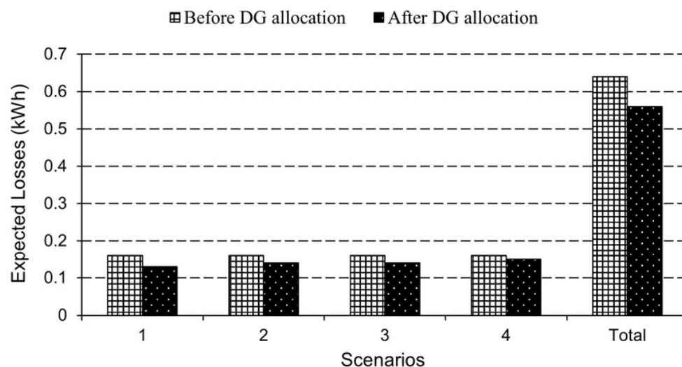
Figure 6. Active power losses for 33-bus network.
