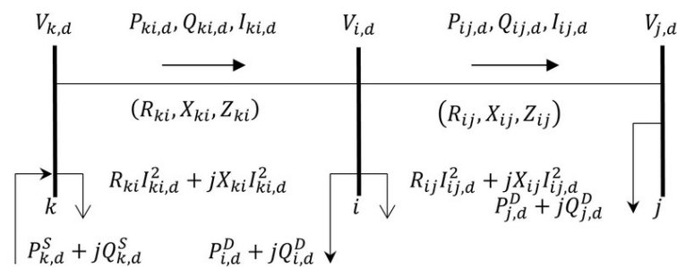
Figure 1. Example network .
