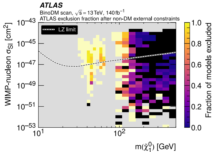
Fig. 21. Fraction of models passing all non-DM external constraints but excluded by ATLAS. The y-axis shows the WIMP–nucleon spin-independent scattering cross-section \sigma_{\text{SI}} , while the x-axis shows the mass of the neutralino LSP m(\tilde{\chi}_1^0) . Bins in grey indicate that no model passes external constraints, while for bins in cream (black) all models are (not) excluded.
