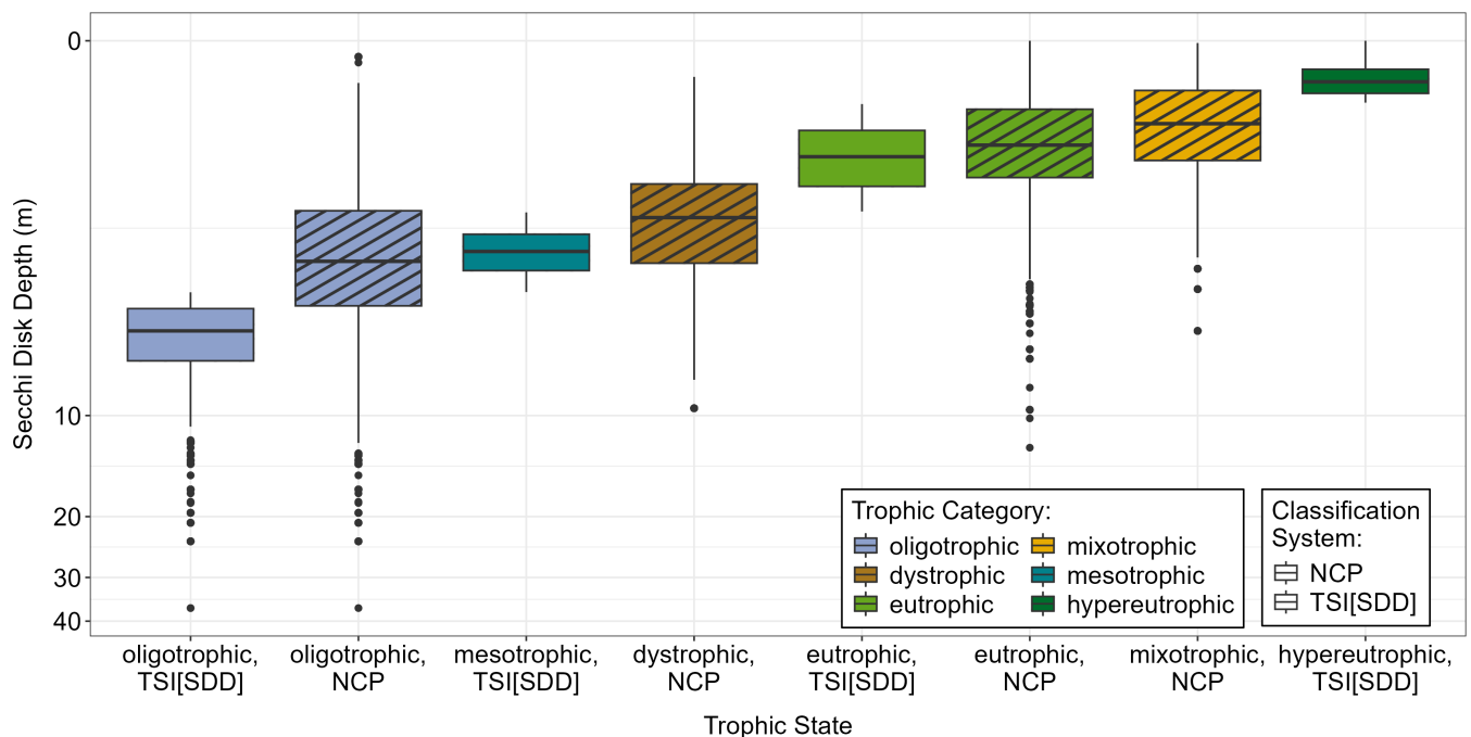
FIGURE 2 Boxplots representing characteristic Secchi disk depths for lakes from the U.S. Environmental Protection Agency (EPA) 2012 and 2017 National Lakes Assessment (NLA) and their associated trophic categories as determined by Nutrient Color Paradigm (NCP) and Trophic State Index (TSI). Boxplots representing NCP-based categories have diagonal hatches, whereas boxplots lacking diagonal hatches represent TSI-based categories. Boxplot lines represent quartile statistics, and points outside lines represent outliers. Secchi disk depth, total phosphorus, and true color data come from the EPA NLA (U.S. Environmental Protection Agency, 2011, 2012, 2017a, 2017b). TSI delineations were made following guidelines in Carlson (1977). NCP delineations were made following thresholds established in Webster et al. (2008) and Leech et al. (2018). Further details on the EPA NLA sampling design are included in Appendix S1. This figure was created using the R script “secchi_depth_boxplots.R” provided in the companion software release (Meyer et al., 2025).
