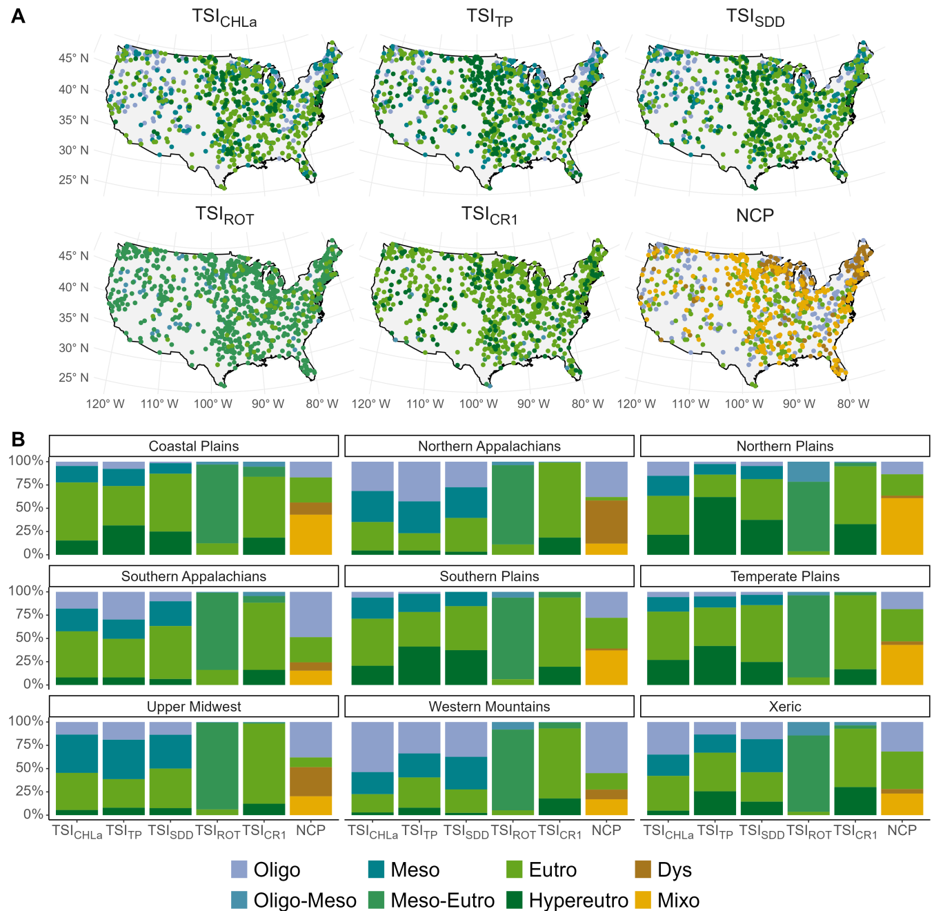
FIGURE 3 (A) Map and (B) aggregated percentages in Omernik Level III aggregated ecoregions of lake trophic state (TS) using various classification schemes. Classification schemes shown here are not necessarily the most common but are intended to reflect the diversity of potential schemes. Notably, TS classifications can produce dramatic differences in anticipated frequency and abundance of a given TS. For example, the Nutrient Color Paradigm (NCP) tends to identify far fewer eutrophic lakes in the Northern Appalachian (3.7% of lakes) and Upper Midwest (10.7%) ecoregions, relative to Trophic State Index (TSI)-based metrics (35.4% and 41% on average, respectively). TS classifications are based on chlorophyll a ( TSI_{CHLa} ), total phosphorus ( TSI_{TP} ), and Secchi disk depth ( TSI_{SDD} ), rotifer abundance ( TSI_{ROT} ; Ejsmont-Karabin, 2012), and crustacean zooplankton abundance ( TSI_{CR1} ; Ejsmont-Karabin & Karabin, 2013), as well as the NCP. Data for trophic state (TS) classifications come from the 2017 U.S. Environmental Protection Agency (EPA) National Lakes Assessment (NLA) sampling campaign (U.S. Environmental Protection Agency, 2017a, 2017b). Further details on the EPA NLA sampling design are included in Appendix S1. This figure was created using the R script “lts_refinement_map.R” provided in the companion software release (Meyer et al., 2025).
