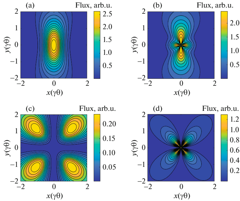
Fig. 2. Spatial angular distribution of \sigma (top) and \pi (bottom) modes for the first harmonic calculated by classical method (left) and in semiclassical approximation (right).
