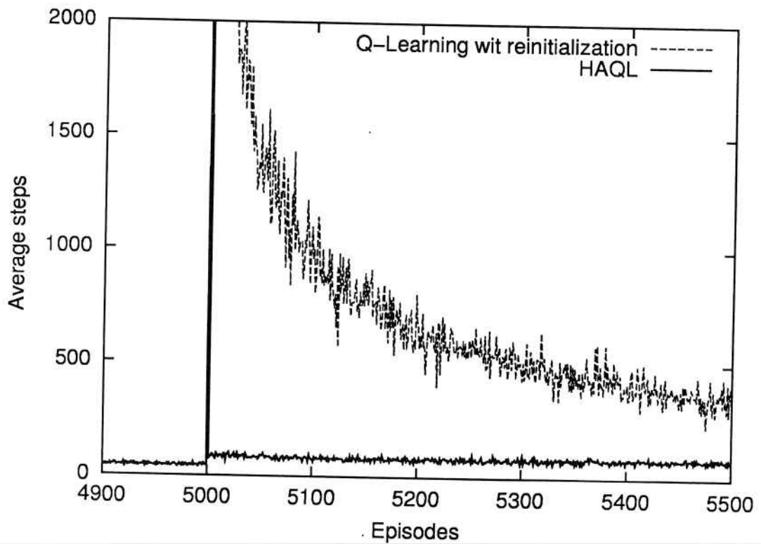
Figure 10: Result for goal repositioning on 5000 th iteration.
