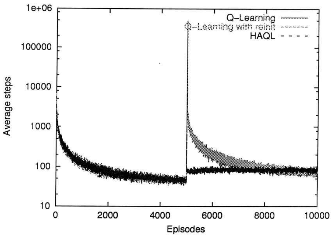
Figura 8: Result for the goal repositioning of 5000 nd iteration (log y).
