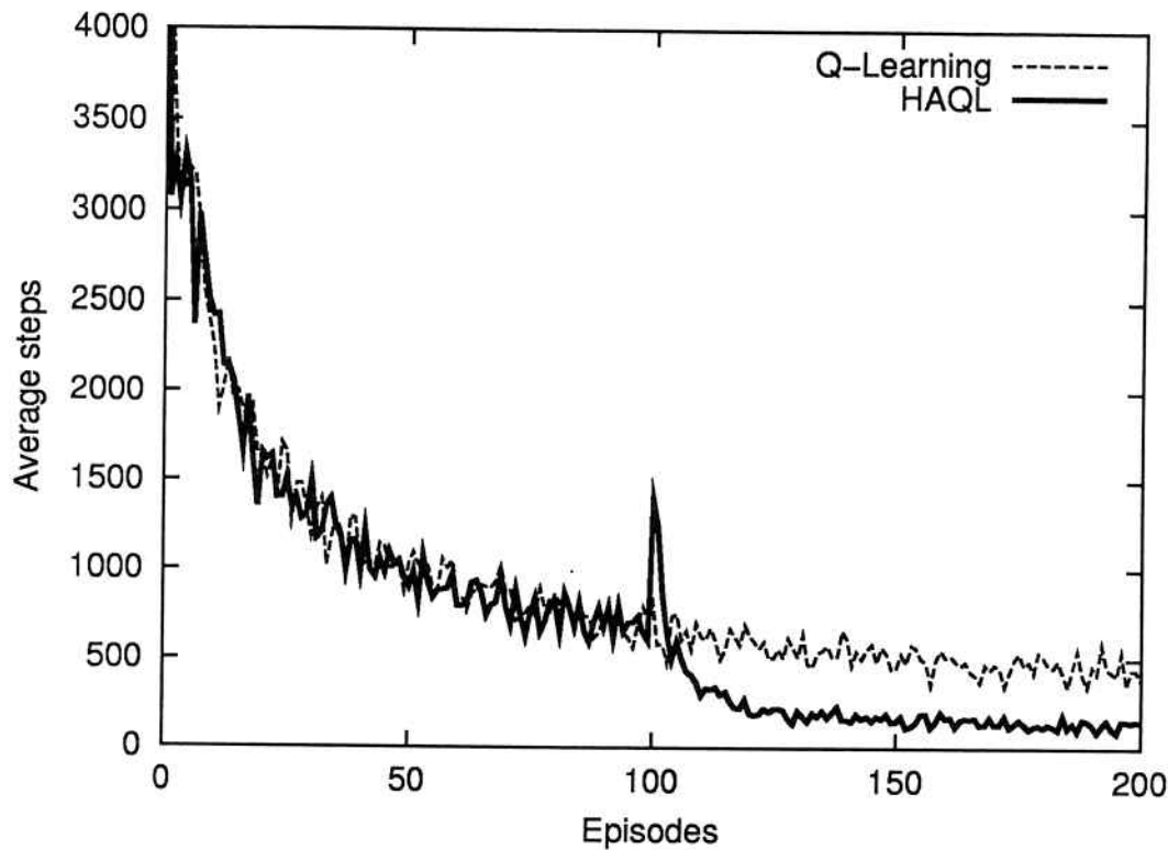
Figure 11: Result for the speedup on 100 th iteration.
