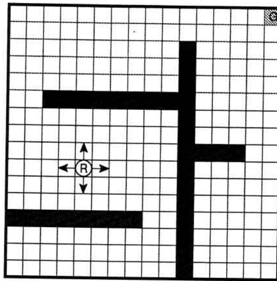
Figure 4: room with walls (represented by dark lines) discretized in a grid of states (represented by softer lines).
