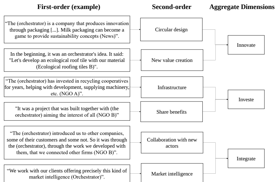
Figure 1. Code tree.
