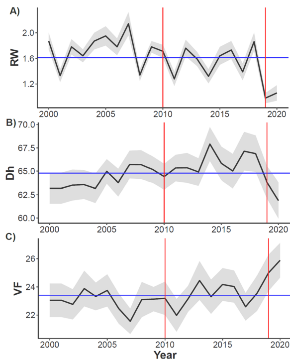
Fig. 3 Annual variation of A tree ring width (RW, mm yr -1 ), B hydraulic diameter ( D_h , \mu m) and C vessel frequency (VF, ind mm -2 ) for the period 2000–2020. The black line is the mean and the shaded area is the standard error. Red vertical lines represent the start of the megadrought in 2010 and the extreme drought in 2019
