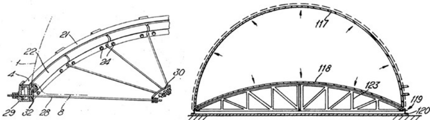
Figure 12. Stiffening of the foundation with the use of a rigid ring. Adapted from [27].
