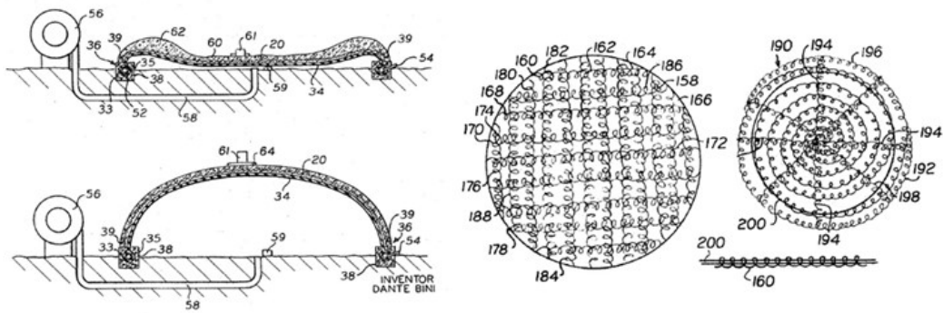
Figure 15. Construction method and disposition of reinforcement in Bini's shells. Adapted from [32].
