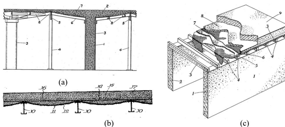
Figure 3. Improvements made by (a) Fletcher [7]; (b) Govan and Ashenhurst [8] and (c) Farrar et al. [9].
