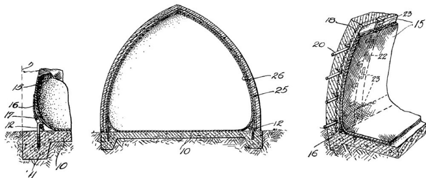
Figure 9. The Neff system for executing shells with inflated membranes. Adapted from [24].
