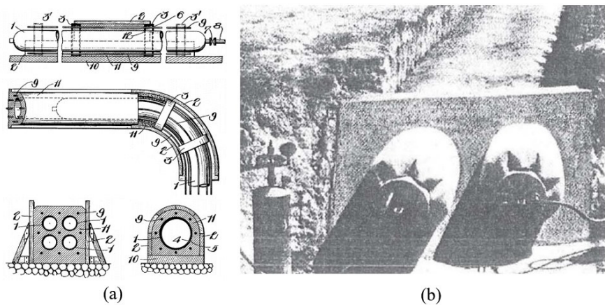
Figure 7. (a) Apparatus for concrete casting pipelines using inflatable tubes –adapted from [19] and (b) construction of a pipeline in Italy in 1938 –adapted from [20].
