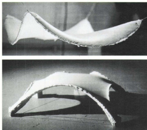
Figure 24. Isler shells generated by suspended fabrics. Adapted from [48].
