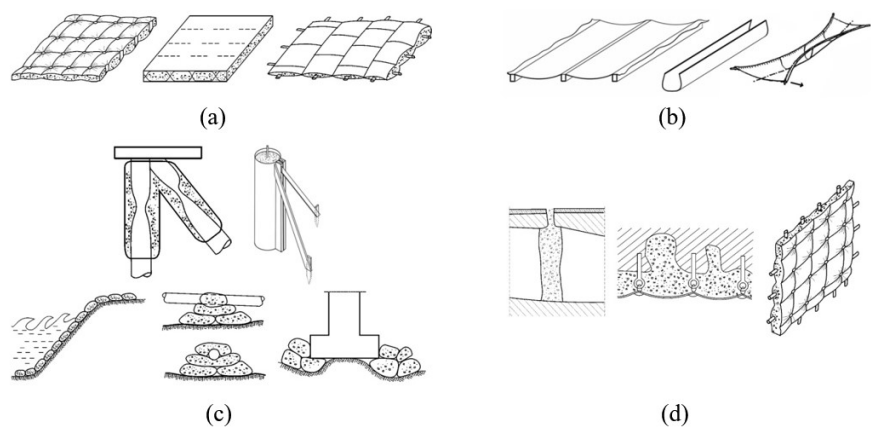
Figure 21. Types of flexible moulds according to Abdelgader et al. [15]: (a) cushion moulds; (b) open moulds; (c) bag-type moulds; (d) covering moulds. Adapted from Abdelgader et al. [15].
