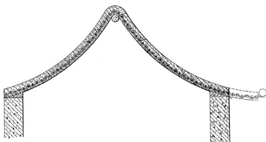
Figure 4. A coverage produced with a fabric mould. Adapted from [10].
