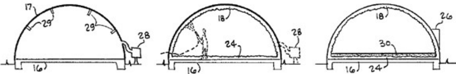
Figure 11. Internal stiffening of the pneumatic casing before the external application of concrete. Adapted from [26].
