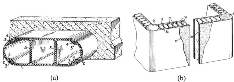
Figure 8. Use of inflated tubes to produce hollow bricks – (a) adapted from [21]; and use of inflated tubes to produce lightweight hollow concrete panels – (b) adapted from [22].
