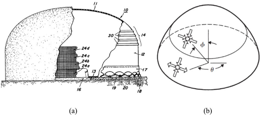
Figure 10. (a) Improvements to Neff system - Adapted from [25] and (b) identification of the horizontal rupture plane, which in the case of spherical shell corresponds to \phi = 51,5^{\circ} - Adapted from [4].
