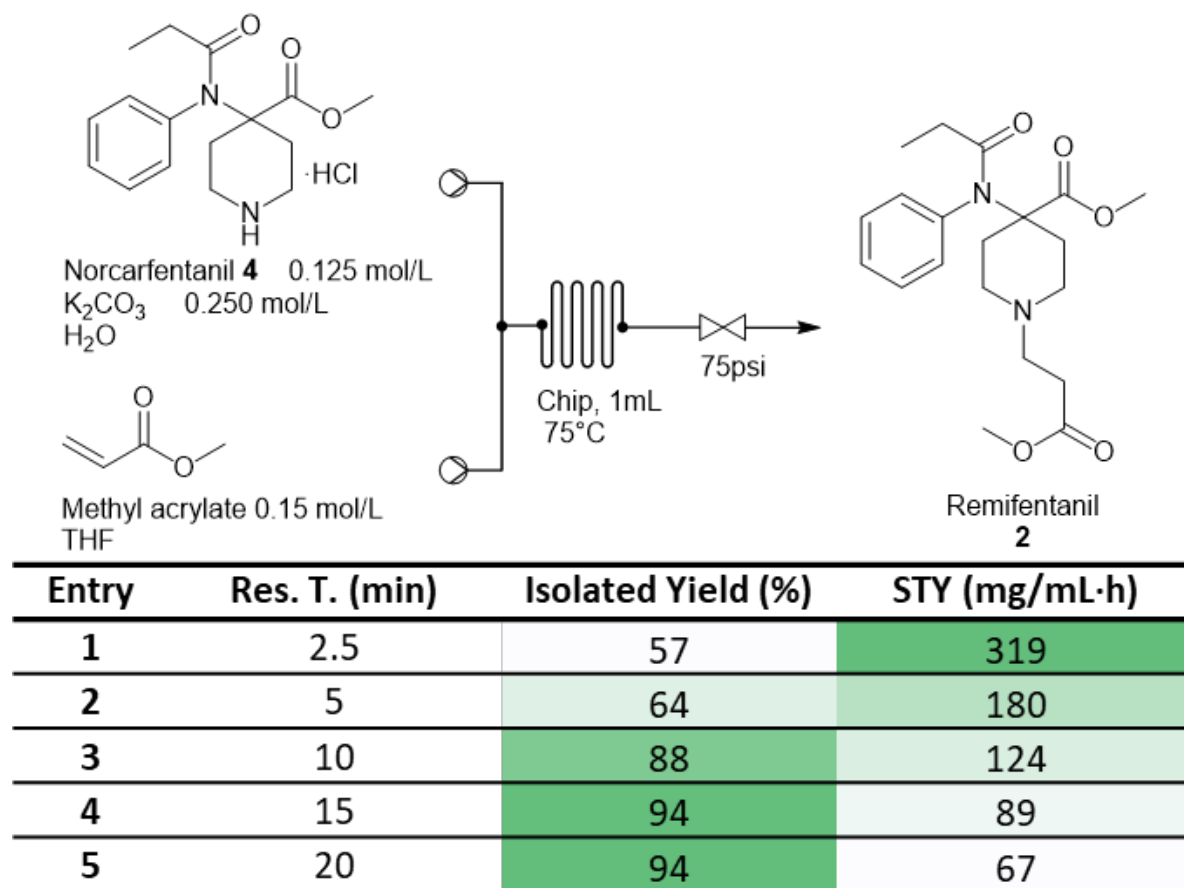
FIGURE 2 - Flow setup diagram for the aza-Michael reaction for preparing remifentanil and space-time yields under different reaction residence times.
