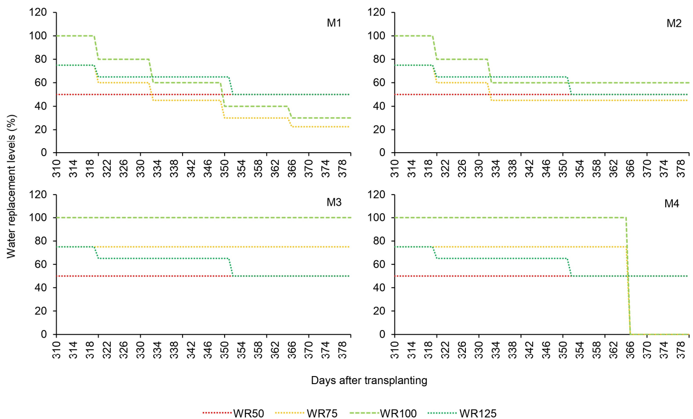
Figure 3. Water replacement levels applied during the sugarcane maturation phase for treatments M1, M2, M3 and M4. The reference irrigation depth is the WR100 treatment for each variety.
