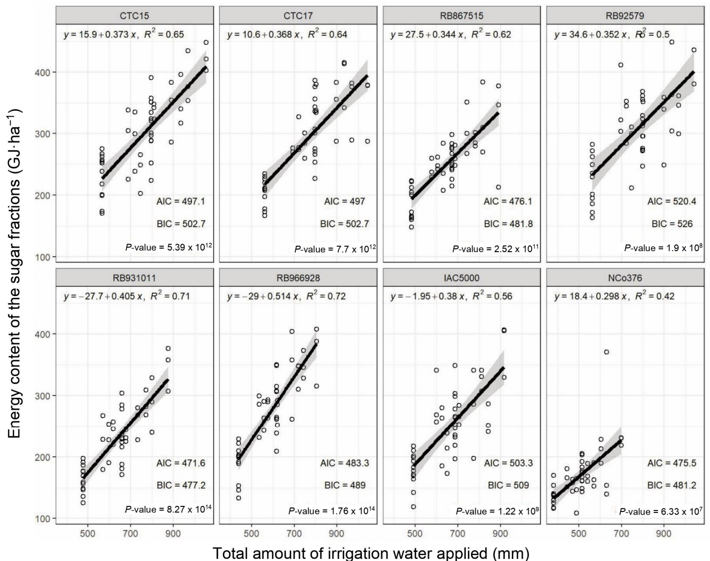
Figure 7. Relationship between the energy content of the sugar fractions for the eight varieties studied and the total amount of irrigation water applied. R^2 : coefficient of determination, AIC: Akaike information criterion, BIC: Bayesian information criterion. The gray shadow represents the confidence interval at the 95% level.
