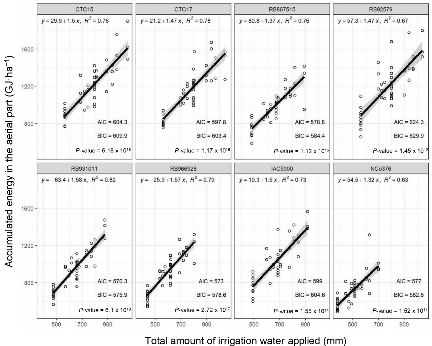
Figure 6. Relationship between accumulated energy in the aerial part of the sugarcane for the eight varieties studied and the total amount of irrigation water applied. R 2 : coefficient of determination, AIC: Akaike information criterion, BIC: Bayesian information criterion. The gray shadow represents the confidence interval at the 95% level.
