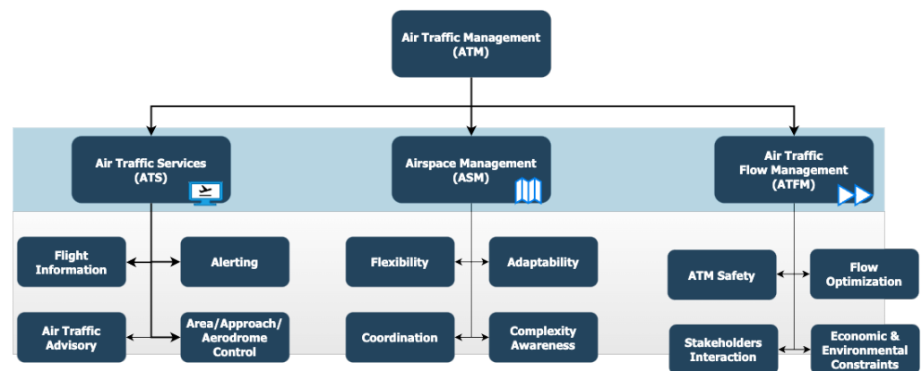
Figure 6. Overview of ATM components [1,26–28].
