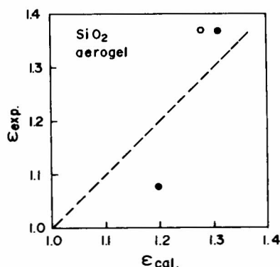
FIGURE 3 Comparison of the measured dielectric constant of neutral gels of different composition ( f = 10 KHz, T = 100 K) with calculated dielectric constant using the Looyenga's relation applied to the first model (○) and to the second structure model (see text).
