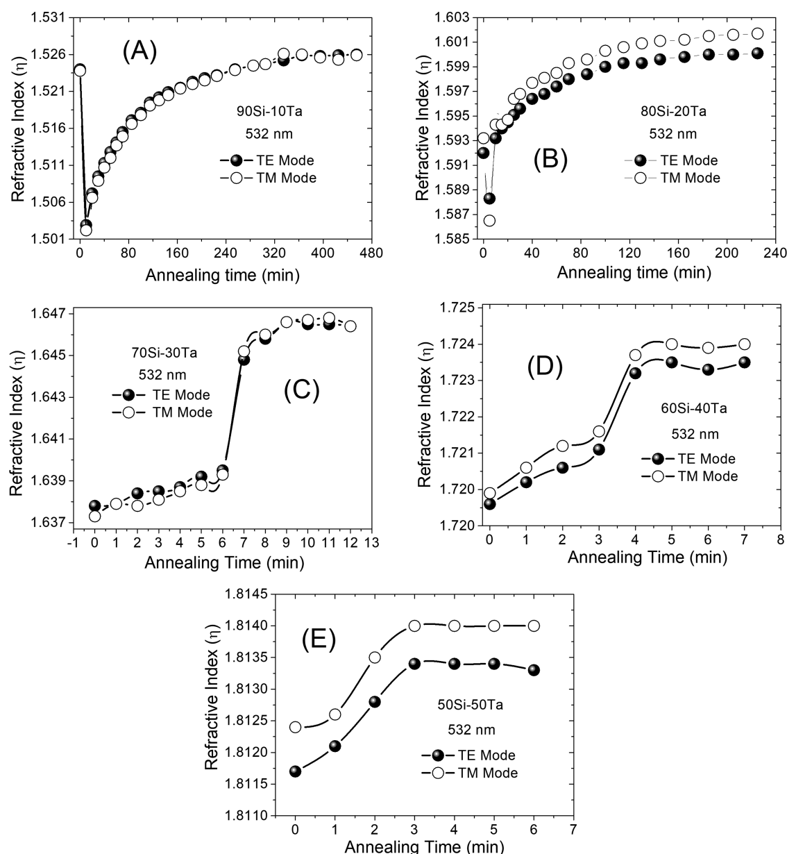
Figure 1. Refractive index values as a function of the annealing time at 900 °C of the \text{Er}^{3+} -doped planar waveguides deposited onto the 10 \mu\text{m} \text{SiO}_2 -Si (100) p-type silicon substrate with Si/Ta ratios of (A) 90:10, (B) 80:20, (C) 70:30, (D) 60:40, and (E) 50:50.
