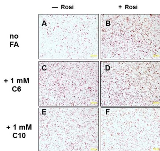
Figure 4. MCFAs that bind PPAR \gamma block TZD-dependent 3T3-L1 cell differentiation. 3T3 fibroblasts were induced to differentiate with Insulin, Dexamethasone and Isobutylmethylxanthine \pm 100 nM rosi (A, C, E versus B, D, F), 1 mM HA C6 (C, D) or 1 mM DA C10 (E, F). Adipogenesis was tested by Red Oil O staining and results showed that DA C10, but not HA C6, is weakly adipogenic and blocks rosi effects. doi:10.1371/journal.pone.0036297.g004
