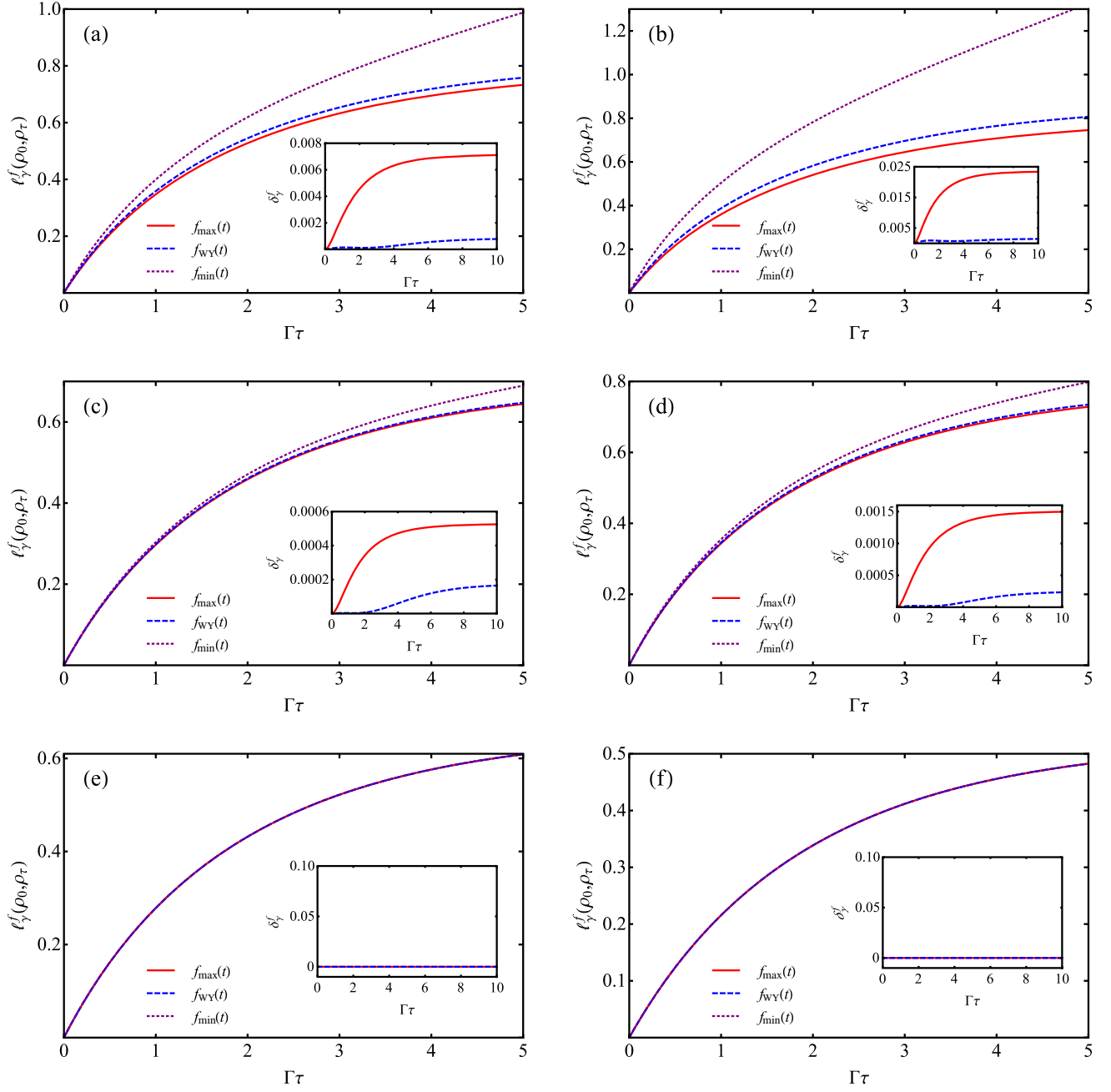
FIG. 6. Evolution path lengths \ell_Y^f for amplitude damping processes related to the contractive Riemannian metrics corresponding to the following MC functions: f_{\text{QF}}(t) = f_{\text{max}}(t) (red solid line), f_{\text{WY}}(t) (blue dashed line), and f_{\text{min}}(t) (purple dotted line) for (a) r_0 = 1/2 , \theta_0 = \pi/2 , (b) r_0 = 3/4 , \theta_0 = \pi/2 , (c) r_0 = 1/4 , \theta_0 = \pi/4 , (d) r_0 = 1/4 , \theta_0 = \pi/2 , (e) r_0 = 1/4 , \theta_0 = 0 , and (f) r_0 = 1/2 , \theta_0 = 0 . The insets in each panel show the relative difference \delta_Y^f , Eq. (19), for amplitude damping processes by considering the quantum Fisher information metric (red solid line) and the Wigner-Yanase information metric (blue dashed line); such a relative difference can be regarded as an indicator of the tightness of the bounds (the smaller \delta_Y^f , the tighter the bounds).
