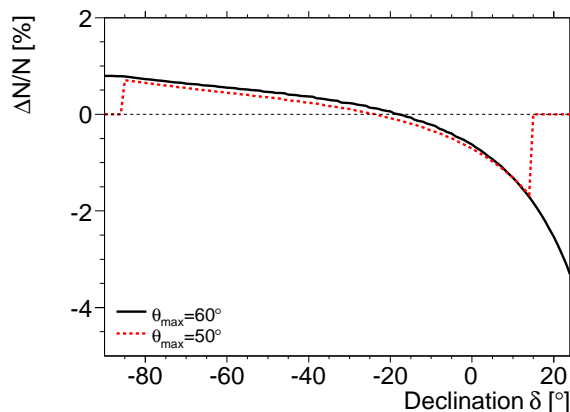
Figure 9. Relative differences \Delta N/N as a function of the declination, for 2 different values of \theta_{\max} .
