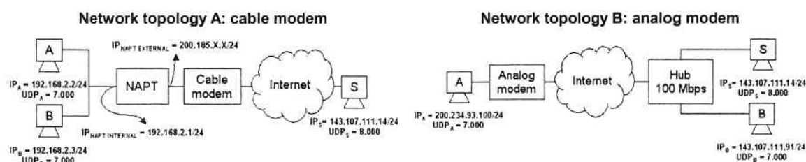
Figure 4. Network topologies for the remote tests.
