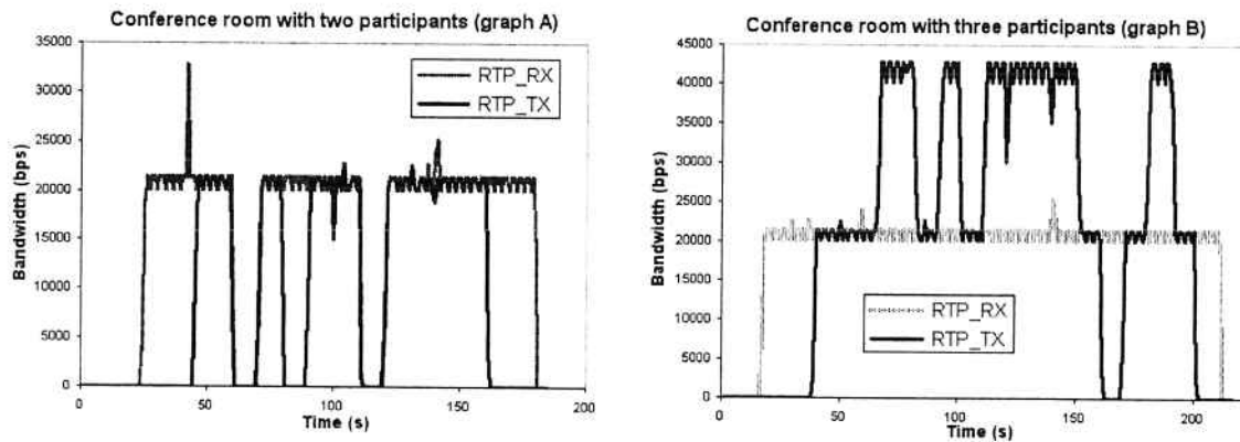
Figure 3. Network bandwidth measured at the multipoint control unit (MCU) in tests #1 (graph A) and #2 (graph B).
