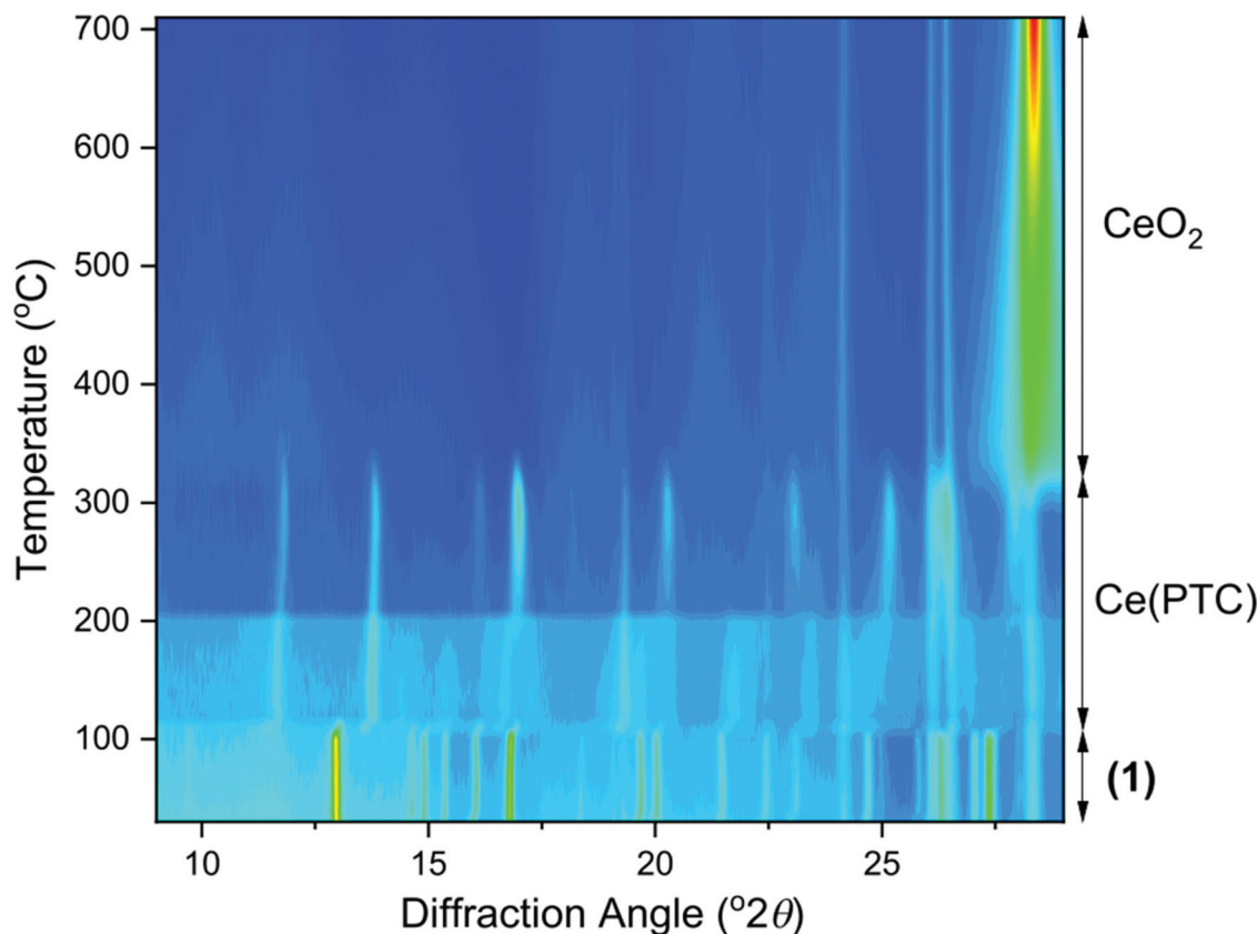
Fig. 8 Thermogravimetric analysis measured for (1) on heating in air, with the phases present indicated.
