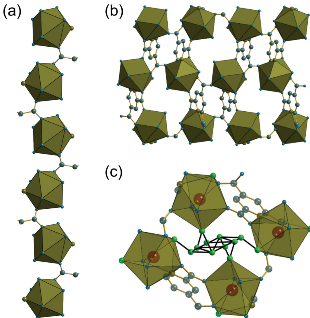
Fig. 2 (a) Chains of nine-coordinate Ce centres found in (1) running parallel to b . (b) Projection of the structure in the ab plane showing connection of chains to yield an open structure (extra-framework water molecules not shown). (c) The local environment of water in (1) with short oxygen–oxygen distances (2.5 to 3 Å) indicative of hydrogen bonding shown in black. Note that the extra framework water sites are not fully occupied so not all will be simultaneously populated. The cerium environment is represented by the polyhedra, and grey spheres are carbon, blue are oxygen, olive are nitrogen and hydrogens are not shown. In (c) the green spheres are the oxygens of water molecules.
