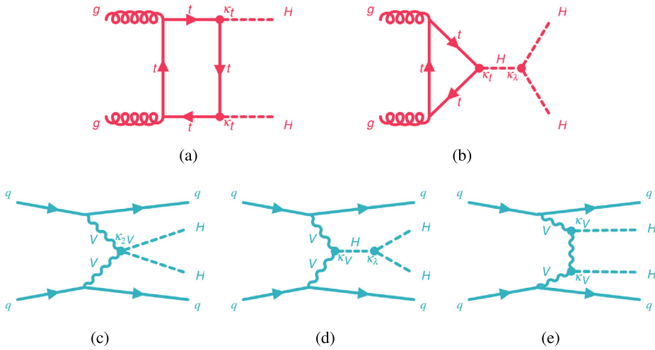
Fig. 2. Examples of leading-order Feynman diagrams for Higgs boson pair production in the (a and b) ggF HH and (c, d and e) VBF HH modes.
