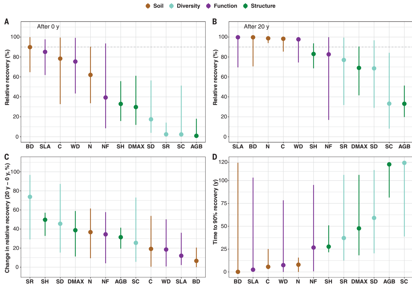
Fig. 3. Relative recovery of SF attributes. (A) Recovery at land abandonment (0 year). (B) Recovery at 20 years. (C) Difference in recovery between 0 and 20 years ( R_{20y} - R_{0y} ). (D) RT until 90% recovery toward OGF values. Relative recovery is expressed as the similarity (in percentage) between the SF value and the OGF value. Medians and 95% credible intervals are based on site predictions;
