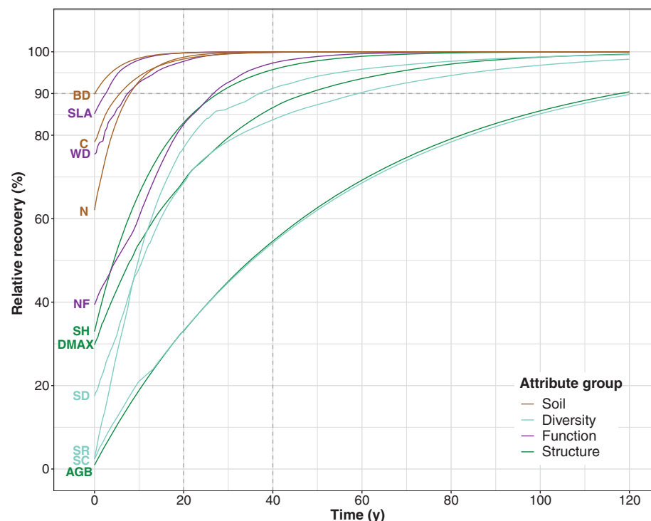
Fig. 2. Predicted relative recovery trajectories over time for 12 forest attributes. The attributes are related to soil (brown), plant functioning (purple), structure (green), and diversity (turquoise). Relative recovery is expressed for each attribute as the similarity (in percentage) between the predicted age-dependent SF value and the OGF value. For some attributes, absolute values increase over time (e.g., AGB), whereas for other attributes, the absolute values generally decrease over time (e.g., BD) (compare Fig. 1A). Here, we show similarity with OGF values, which, by definition, increases over time (compare Fig. 1B). Succession often starts with some remnant trees and soil legacies, and some attributes (SLA and WD) can never be zero, which explains why most attributes do not start at zero (see main text). Dashed lines indicate relative recovery at 20 years, recovery at 40 years, and RT until 90% recovery toward OGF values (see Fig. 3). Recovery trajectories are across-site median values were estimated by using Bayesian models for each attribute (see supplementary text S1). C, soil C; N, soil N; NF, proportional basal area of nitrogen-fixing species; SLA, community-weighted mean SLA; WD, community-weighted mean WD.
