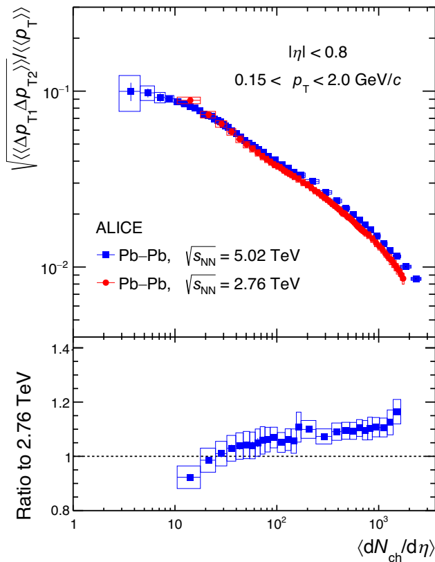
Fig. 4 (top) Normalized transverse momentum correlator, \sqrt{\langle\langle\Delta p_{T1}\Delta p_{T2}\rangle\rangle}/\langle\langle p_T\rangle\rangle , shown as a function of the charged-particle multiplicity density, \langle dN_{ch}/d\eta\rangle , in Pb–Pb collisions at \sqrt{s_{NN}} = 2.76 [23] and 5.02 TeV; (bottom) Ratio of values of \sqrt{\langle\langle\Delta p_{T1}\Delta p_{T2}\rangle\rangle}/\langle\langle p_T\rangle\rangle measured at \sqrt{s_{NN}} = 5.02 TeV to the corresponding results at \sqrt{s_{NN}} = 2.76 TeV. The statistical and systematic uncertainties for both energies are represented by vertical bars and boxes, respectively
