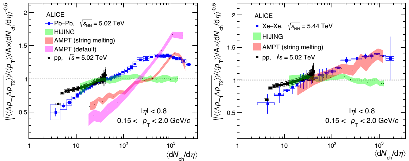
Fig. 3 Evolution of the ratio of \sqrt{\langle \Delta p_{T1} \Delta p_{T2} \rangle} / \langle p_T \rangle to results of a power-law fit to HIJING calculations: (left) pp and Pb–Pb collisions at \sqrt{s_{NN}} = 5.02 TeV; (right) pp collisions at \sqrt{s_{NN}} = 5.02 TeV and Xe–Xe collisions at \sqrt{s_{NN}} = 5.44 TeV. The power-law fit was performed on correlator values obtained with HIJING for Pb–Pb collisions at \sqrt{s_{NN}} = 5.02 TeV and Xe–Xe collisions at \sqrt{s_{NN}} = 5.44 TeV for left and
