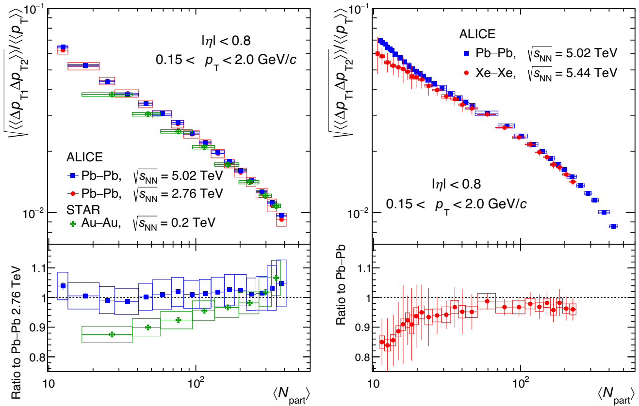
Fig. 5 Left: normalized transverse momentum correlator, \sqrt{\langle\langle\Delta p_{T1}\Delta p_{T2}\rangle\rangle}/\langle\langle p_T\rangle\rangle , shown as a function of the average number of participant nucleons, \langle N_{part}\rangle , in Pb–Pb collisions at \sqrt{s_{NN}} = 2.76 and 5.02 TeV and Au–Au collisions at 0.2 TeV. Right: normalized
