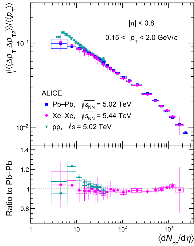
Fig. 1 (top) Normalized transverse momentum correlator, \sqrt{\langle\Delta p_{T1}\Delta p_{T2}\rangle}/\langle p_T\rangle , shown as a function of the charged-particle multiplicity density, \langle dN_{ch}/d\eta\rangle , measured in the pseudorapidity range |\eta| < 0.8 in pp collisions at \sqrt{s} = 5.02 TeV, Xe–Xe collisions at \sqrt{s_{NN}} = 5.44 TeV, and Pb–Pb collisions at \sqrt{s_{NN}} = 5.02 TeV; (bottom) Ratio of values of \sqrt{\langle\Delta p_{T1}\Delta p_{T2}\rangle}/\langle p_T\rangle measured in pp and Xe–Xe collisions to those observed in Pb–Pb collisions. Statistical and systematic uncertainties are represented by vertical bars and boxes, respectively
