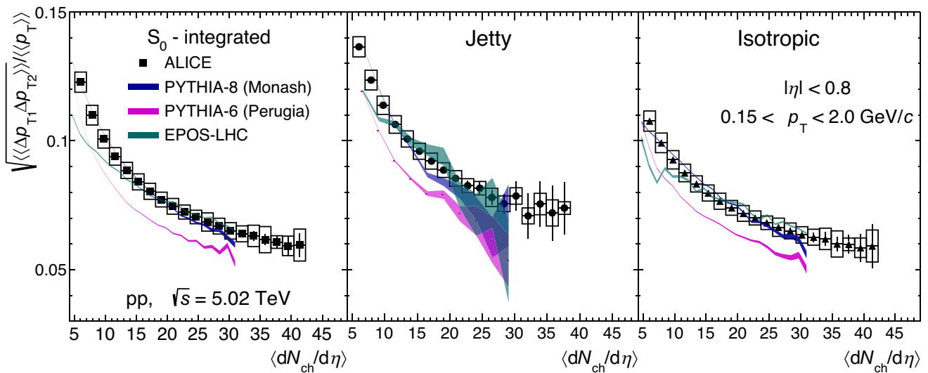
Fig. 8 Comparison of normalized transverse momentum correlator, \sqrt{\langle\langle\Delta p_{T1} \Delta p_{T2}\rangle\rangle} / \langle\langle p_T \rangle\rangle as a function of the produced particle multiplicity for integrated (left), jetty (middle), and isotropic (right) pp collisions at \sqrt{s} = 5.02 TeV with calculations from the PYTHIA and EPOS mod-
