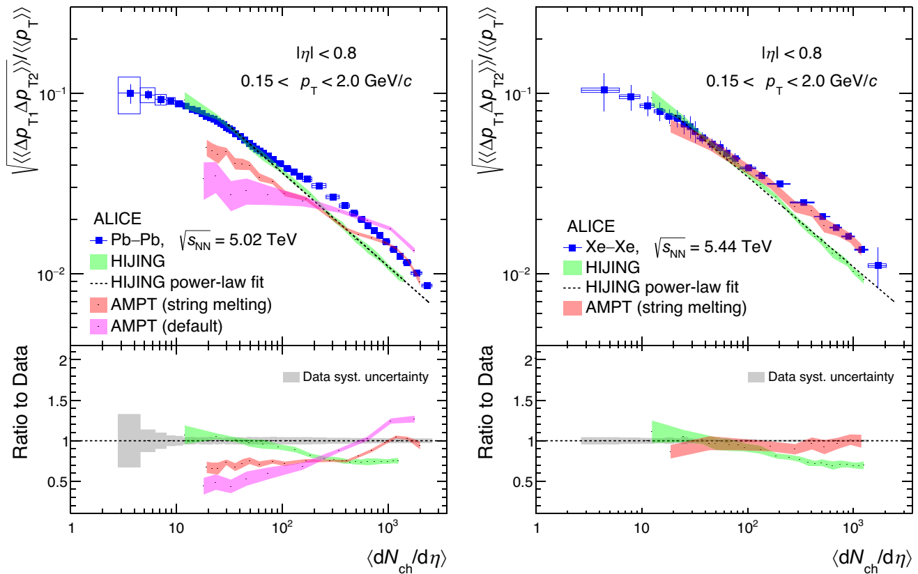
Fig. 2 Upper panels: comparisons of the evolution of the strength of \sqrt{\langle\langle\Delta p_{T1}\Delta p_{T2}\rangle\rangle/\langle p_T\rangle} with produced charged-particle multiplicity densities, \langle dN_{ch}/d\eta\rangle , in Pb–Pb collisions at \sqrt{s_{NN}} = 5.02 TeV (left) and Xe–Xe collisions at \sqrt{s_{NN}} = 5.44 TeV (right) with calculations using the HIJING and AMPT models. Lower panels: ratios of the model cal-
