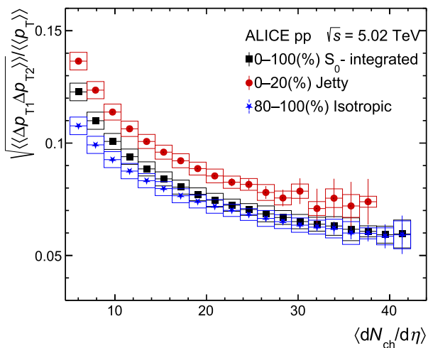
Fig. 6 Comparison of the normalized transverse momentum correlator, \sqrt{\langle\langle\Delta p_{T1}\Delta p_{T2}\rangle\rangle}/\langle\langle p_T\rangle\rangle as a function of the charged-particle multiplicity density for sphericity-integrated (black), jetty (red), and isotropic (blue) events in pp collisions at \sqrt{s} = 5.02 TeV. The statistical and systematic uncertainties of the measured data for all sphericity classes are represented by vertical bars and boxes respectively
