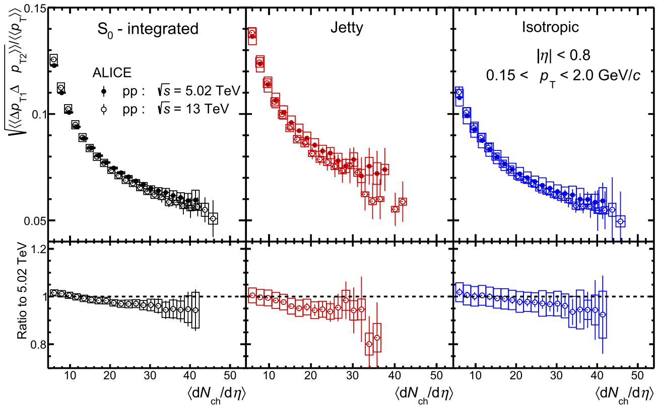
Fig. 7 Upper panels: comparison of the normalized transverse momentum correlator, \sqrt{\langle\langle\Delta p_{T1} \Delta p_{T2}\rangle\rangle} / \langle\langle p_T \rangle\rangle as a function of charged-particle density in pp collisions at \sqrt{s} = 5.02 and \sqrt{s} = 13 TeV for sphericity-integrated (left), jetty (middle) and isotropic (right) events; Lower pan-
