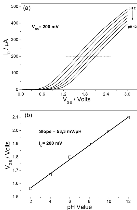
Figure 6. I_D - V_{GS} characteristics for constant V_{DS} of the ITO film as separate extend gate-FET in the pH range from 2 to 12: (a) I_D - V_{GS} characteristics, and (b) sensitivity calculated when I_D was fixed in 200 \mu A .
