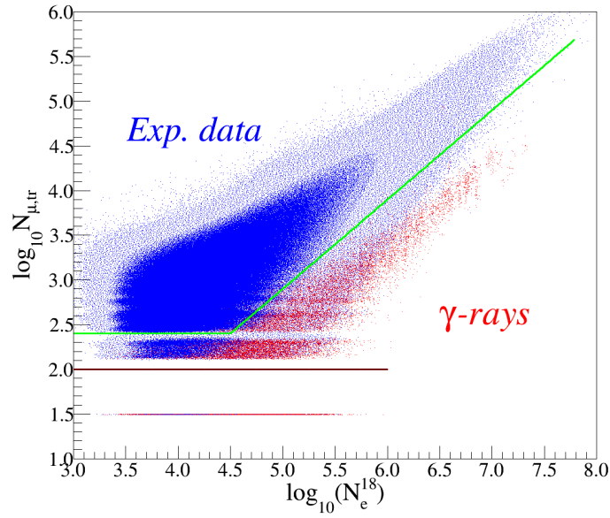
Figure 1: Scatter histogram of the measured number of muons \lg(N_\mu) and number of electrons \lg(N_e) (blue) superimposed with simulated gamma-ray showers (red). The green line indicates the choice of the cut for the selection of the muon-poor showers.
