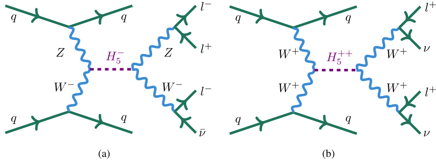
Fig. 1. Representative Feynman diagrams of production and decay of the (a) H_5^\pm and (b) H_5^{\pm\pm} states.
