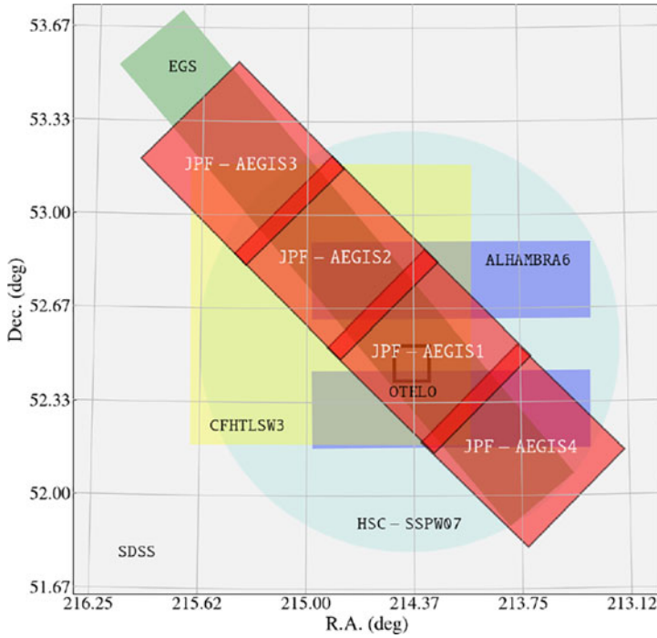
Figure 2. Footprint of the miniJPAS field, with individual pointings shown as red squares. The footprints of other projects are also shown.
