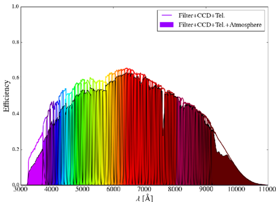
Figure 1. The measured transmission curves for the J-PAS filter set before and after accounting for sky absorption. Effects of the CCD quantum efficiency and the entire optical system of the JST/T250 telescope are included.
