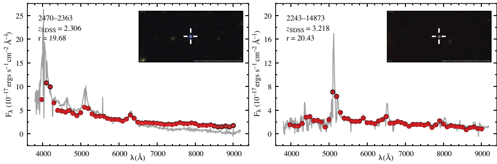
Figure 3. Two examples of SDSS quasar spectra (gray lines) as observed with miniJPAS (red points).
