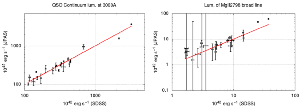
Figure 5. Comparison between the spectral quantities estimated on the SDSS spectra and on the corresponding miniJPAS pseudospectra, as obtained with the QSFIT software. Left panel: QSO continuum luminosity at 3000 Å. Right: integrated luminosity of the MgII emission line.
