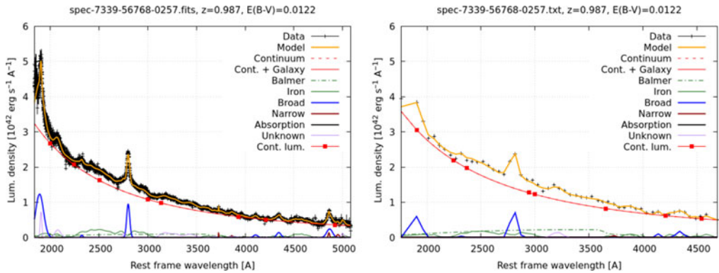
Figure 4. An example of the best fit spectral model obtained running the QSFIT software on a SDSS data (left panel) and on the corresponding low-resolution miniJPAS spectrum (right panel) of a z \sim 1 quasar. The data (black points) and the overall model (orange lines) are shown, together with the contributions of the different components, from the continuum (dashed red lines) to the broad line components (blue lines), as reported in the legend.
