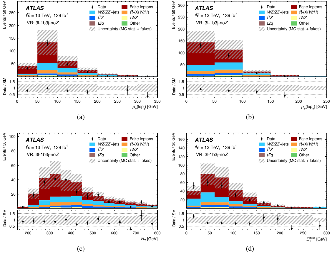
Figure 12. Comparisons of the predicted and observed yields in VR-3 \ell -1 b3j -noZ, with respect to the p_T of the (a) leading and (b) subleading lepton candidates, (c) the scalar sum of the lepton and jet transverse momenta, H_T , and (d) the missing transverse momentum in the event, E_T^{\text{miss}} . The processes with three real leptons are modelled with MC simulation, while the contribution from fake/non-prompt leptons (dark red) comes from the Poisson likelihood matrix method as described above. The hatched band shows the uncertainty from MC statistics and the fake/non-prompt background estimate. The rightmost (leftmost) bins are inclusive and contain all events above (below) the x -axis ranges. The lower panel shows the ratio of data to the total SM prediction (sum of the real-lepton background contributions estimated with MC samples and the fake/non-prompt lepton contribution estimated with the matrix method). Further details are available in ref. [46].
