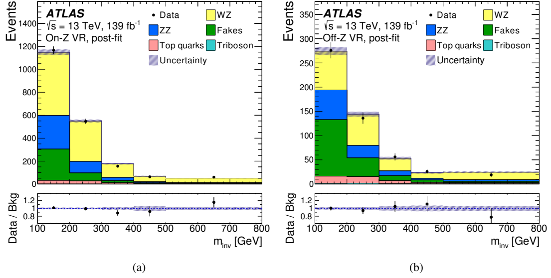
Figure 16. Comparison between data and prediction for the m_{\text{inv}} distribution in the (a) on-Z and (b) off-Z validation regions, after fitting the normalisation factors for the WZ + jets and ZZ + jets backgrounds and systematic uncertainties [48]. All uncertainties, systematic and statistical, are included. The leftmost (rightmost) bin is inclusive and contains all events with m_{\text{inv}} < 200 \text{ GeV} ( > 500 \text{ GeV} ). The hatched grey area in these figures shows the total uncertainty. Further details are available in ref. [48].
