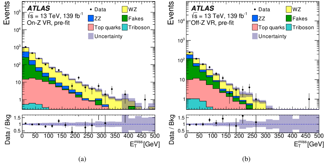
Figure 17. Comparison between data and prediction for the E_T^{\text{miss}} distribution in the (a) on-Z and (b) off-Z validation regions. All uncertainties, systematic and statistical, are included. The rightmost bin is inclusive and contains all events with E_T^{\text{miss}} > 475 \text{ GeV} . The hatched grey area in these figures shows the total uncertainty. Further details are available in ref. [48].
