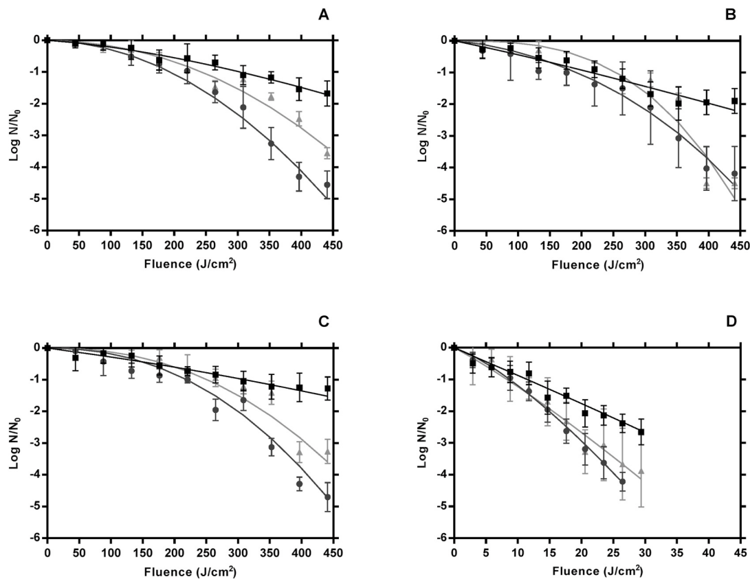
Fig. 4. aPDT inactivation curves of the spores of different strains of B. cereus – B63 (A), 436 (B), B3 (C), and ATCC 14579 (D) – in the presence of NMB at concentrations of ■ 5, ● 50, and ▲ 100 \mu\text{M} and different fluences ( \text{J}/\text{cm}^2 ). All data correspond to three independent experiments. —: estimated curve by the Weibull model. Error bars represent the standard deviation (SD) of three independent experiments and, in some cases, are hidden by the symbols.
