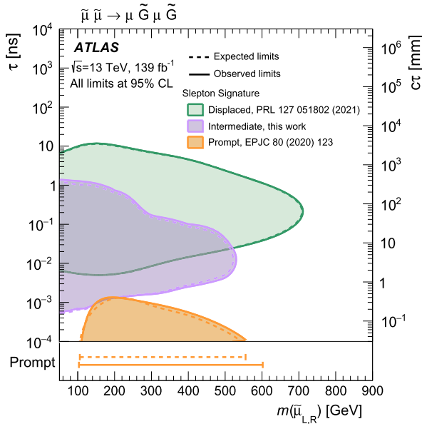
Fig. 4. Expected (dashed) and observed (solid) exclusion contours for \tilde{\mu} NLSP production as a function of the left- and right-handed smuons, \tilde{\mu}_{L,R} , mass and lifetime at 95% CLs, for the Displaced Slepton Signature (Phys. Rev. Lett. 127 051802 (2021) [24]), the Intermediate Slepton Signature (the result of this search in this paper) and the Prompt Slepton Signature (Eur. Phys. J. C 80 (2020) 123 [52]) reinterpretation. The lines below the graphs show the expected and observed limits from the prompt search where the smuons are assumed to be prompt.
