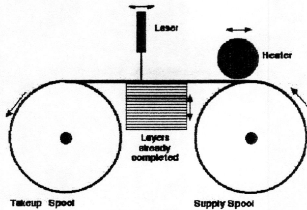
Figure 4 – The LOM process
