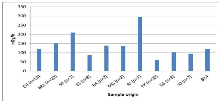
Figure 9: Absorbed dose rate, in nGy h -1 , according to the samples origin (this study: CH, BR1, SP, ES, BA, MG and RJ) and literature values (PK, EG, JO and BR4)
