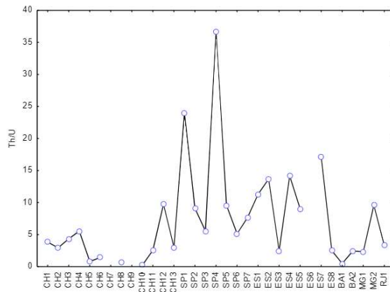
Figure 3: Th/U ratio in the analyzed samples
