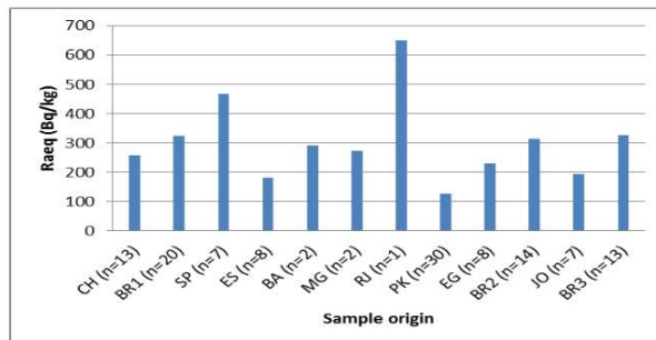
Figure 7: Radium equivalent, in \text{Bq kg}^{-1} , according to the samples origin (this study: CH, BR1, SP, ES, BA, MG and RJ) and literature values (PK, EG, BR2, JO and BR3)
