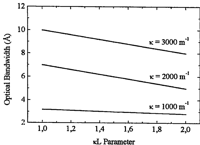
Fig. 4 - Optical filter bandwidth as a function of the \kappa L parameter
