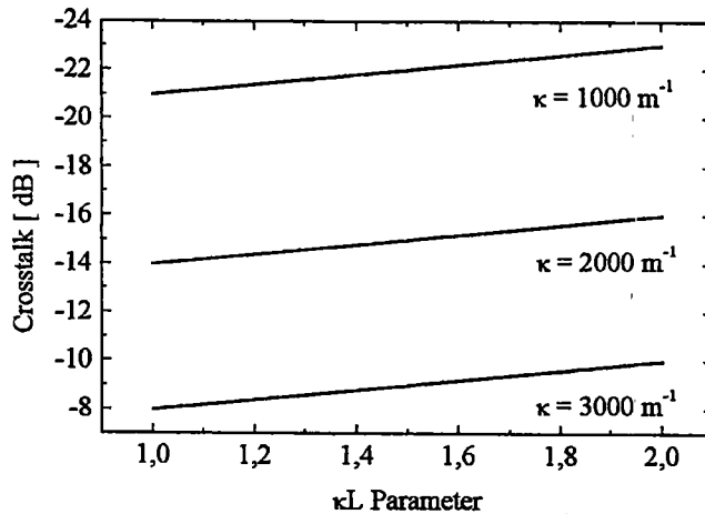
Fig. 5 - Calculated crosstalk plotted as a function of \kappa L parameter. The indicated crosstalk refers only to the dominant next neighbor.
