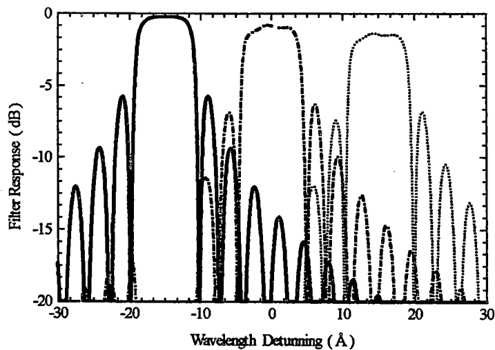
Fig. 3 Filter response. Solid lines represent the first section response, the dashed ones show the response of the second section and the dotted lines show the third filter response.
