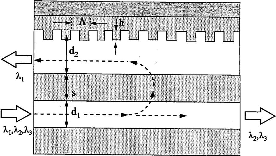
Fig. 1 Cross sectional view of one block of complete filter structure.
