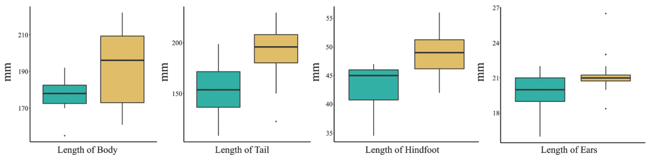
Figure 5. Boxplot showing the descriptive statistics for the external variables explaining the morphometric differences between Pampas (yellow) and Atlantic Forest (green) biomes.
