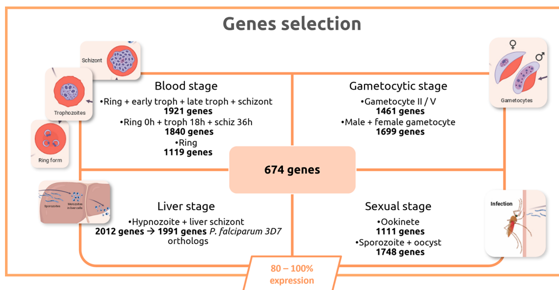
Figure 2. Overlap of highly expressed genes in transcriptomes of different life stages of P. falciparum .
