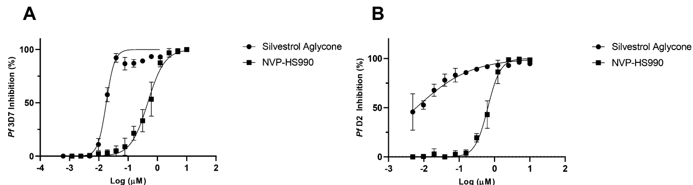
Figure 5. In vitro antimalarial activity of selected compounds against P. falciparum . (A) Inhibition curves of silvestrol aglycone and NVP-HSP990 against chloroquine sensitive (3d7) and (B) multidrug-resistant (Dd2) P. falciparum strains.
