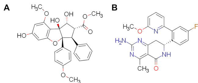
Figure 4. 2D-structure representation of (A) silvestrol aglycone and (B) NVP_HSP990.
