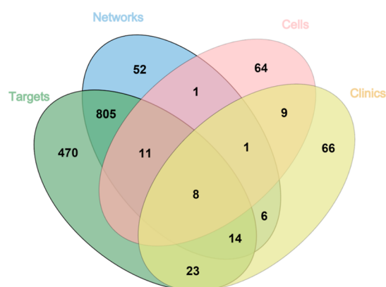
Figure 3. Venn diagram showing the 1557 similar compounds in different bioactivity profiles found using the Chemical Checker database. 18
