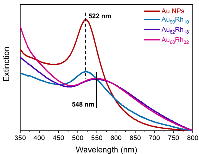
Figure 2. Extinction spectra obtained from aqueous suspensions containing Au NP seeds and from Au 90 Rh 10 , Au 82 Rh 18 , and Au 68 Rh 32 NFs.
