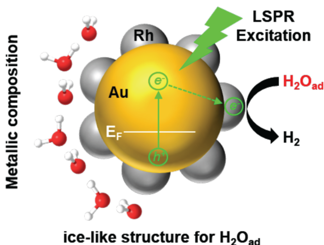
Figure 7. Schematic representation of electron transfer pathways that lead to an enhancement in the HER performances following the LSPR excitation in the Au@Rh NFs. Under 533 nm excitation, hot electrons generated from the Au LSPR excitation can flow to the Rh surface, where they can contribute to the activation of adsorbed \text{H}_2\text{O} species, leading to a decrease in the overpotential.
