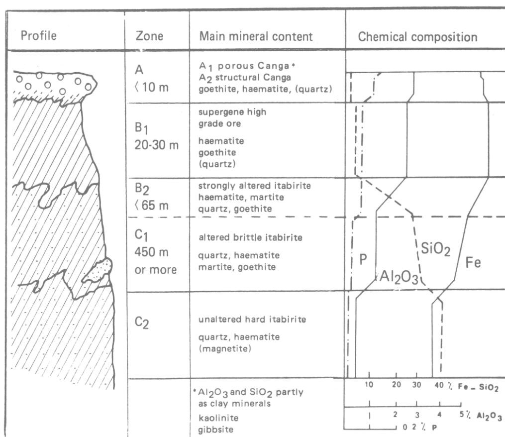
Fig. 10 — Chemical and mineralogical composition along a typical schematic itabirite alteration profile. Quadrilatero Ferrifero (modified after EICHLER, 1967).
