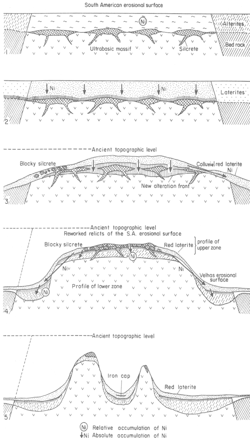
Fig. 14 — Schematic sequence of the different morphotectonic phases of the evolution of the Ni ore deposits in Central Brazil.
