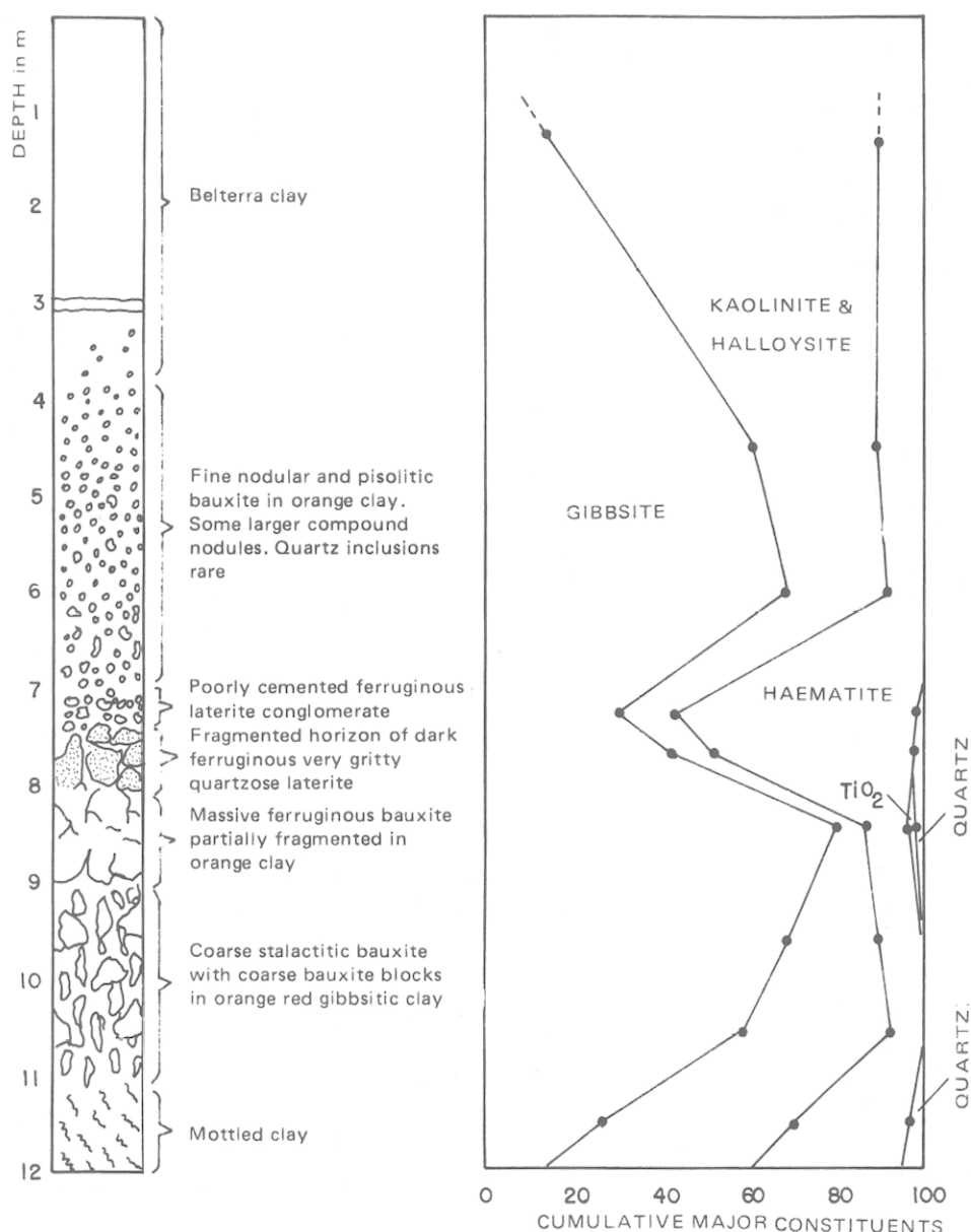
Fig. 8 — Profile section through Trombetas bauxite deposit (after GRUBB, 1979).
