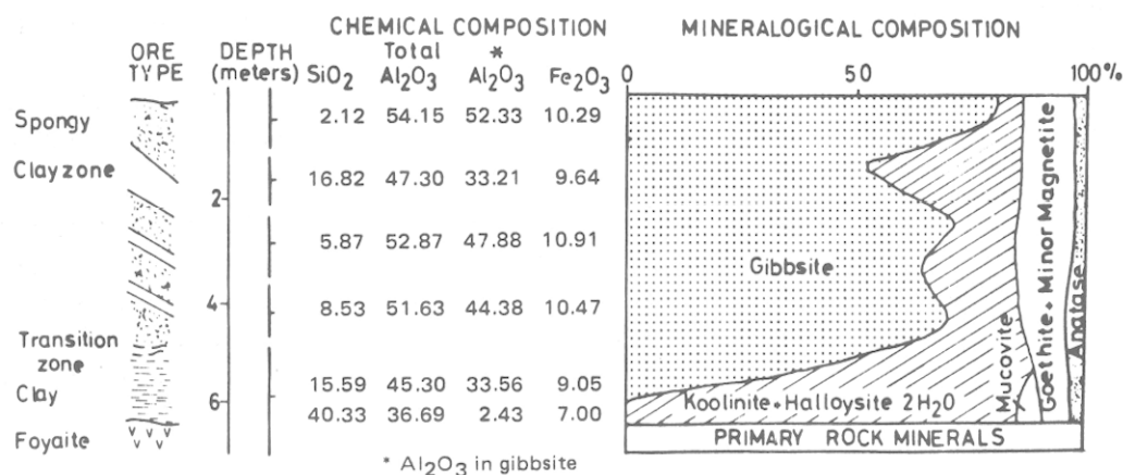
Fig. 5 — Chemical and mineralogical composition along the bauxitic high plateau alteration profiles, Poços de Caldas (after ALMEIDA, 1977).
