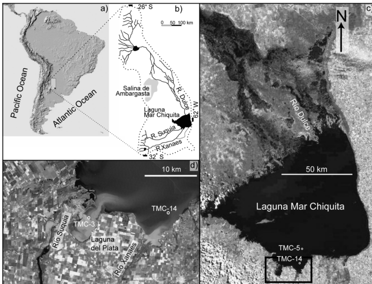
Fig. 1. (a) Geographical map of South America showing the location of Laguna Mar Chiquita in the Pampean plains of Argentina. (b) Detail of the drainage basin. (c) Core location in the satellite image of the lake. (d) Detail of the area indicated in (c) showing the Laguna del Plata with core location.
