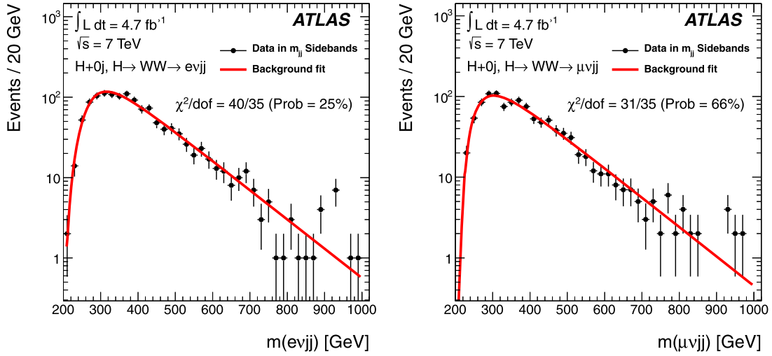
Fig. 1. Fits of the background model described in the text to the reconstructed invariant mass m(\ell v jj) when m_{jj} is in the W sidebands for the \ell v jj + 0j selection. The left (right) figure shows the electron (muon) channel distribution. The \chi^2/\text{dof} and \chi^2 probability of these fits are also shown in the figure.
