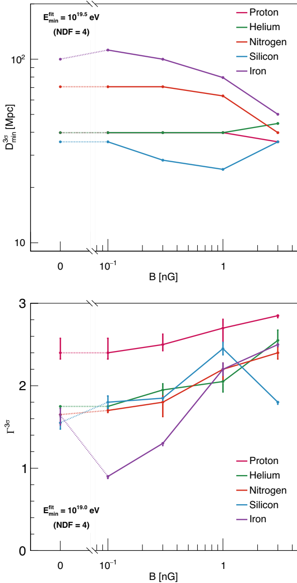
FIG. 8. The top panel shows the evolution of the restrained distance to nearest source, D_{\min}^{3\sigma} , with relation to the field strength, B , while the bottom one shows the evolution of the fitted spectral index, \Gamma , with relation to B . The pink, green, orange, cyan and purple lines represent, respectively, the scenarios with pure proton, helium, nitrogen, silicon, and iron composition at the sources.
