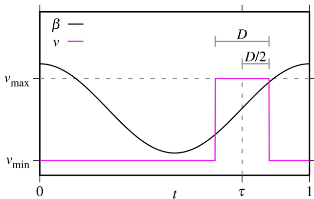
FIG. 10. Schematic illustration of pulsed width vaccination. Transmissivity \beta(t) (black curve) superimposed by vaccination rate v(t) (magenta curve), it is on two levels: maximum v_{\max} (dashed gray line level) and minimum v_{\min} . Pulse width D centered on \tau , which is a time instant relative to the seasonal cycle.
