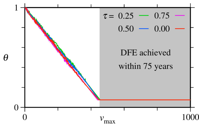
FIG. 8. \theta as a function of v_{\max} \in [0, 1000] from four variants of the pulsed vaccination strategy and obtained in the first 75 years of infection. Horizontal axis discretized in 1001 equidistant points. We consider b = 0.02 , \beta_0 = 270 , \beta_1 = 0.28 , \delta = 0.25 , \alpha = 100 , \gamma = 100 , \omega = 2\pi , and p = v_{\min} = 0 . Initial condition (s_0, e_0, i_0) = (0.9, 0, 0.1) . Pulse application timing identified in colors, according to the legend. DFE is achieved (gray background) within 75 years for v_{\max} \geq 452 with \tau \in [0, 0.5] , v_{\max} \geq 459 for \tau = 0.25 , and v_{\max} \geq 444 when \tau = 0.75 .
