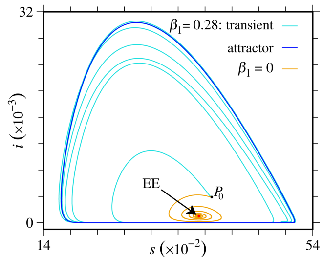
FIG. 2. Trajectories evolving from the initial condition P_0(s_0, e_0, i_0) = (0.39, 0.0039, 0.0039) (black dot). We consider the parameters: v = 0.17 , \lambda = 1 , p = 0.25 , b = 0.02 , \beta_0 = 270 , \delta = 0.25 , \alpha = 100 , and \gamma = 100 . For \beta_1 = 0 , the trajectory (orange line) spirals toward the attractive fixed point EE ( 0.371, 0.001, 0.001 ) (red dot). In the non-autonomous case ( \beta_1 = 0.28 and \omega = 2\pi ), the system evolves (light-blue line) around the point EE converging to the periodic attractor (blue line).
